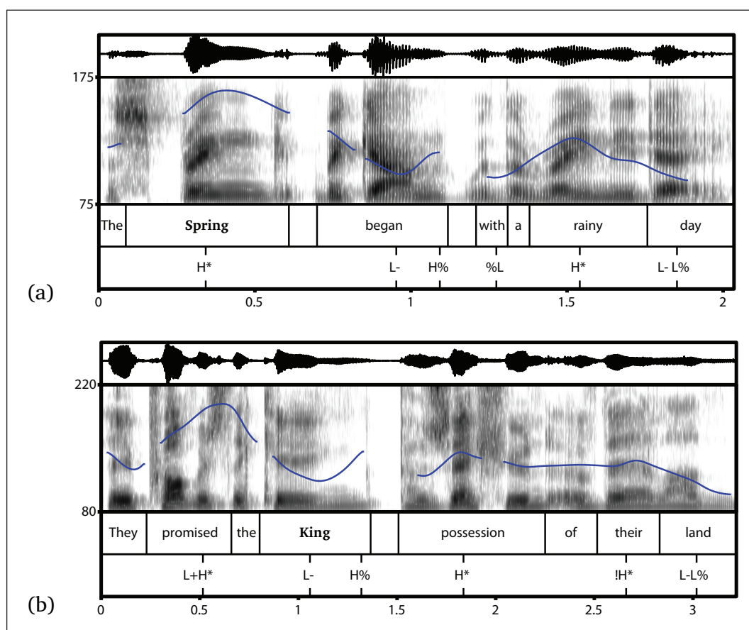
Figure 6: Pitch contours and ToBI annotation for two pre-pausal tokens in the IP-medial context: one genuinely IP-medial in (a) and one produced with phrase-final intonation in (b) .
