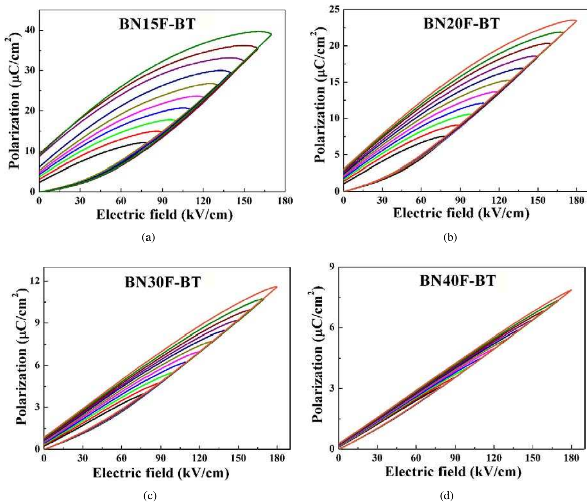
Fig. 33. Unipolar P - E loops under different electric fields for Nd doped 0.75\text{BF-}0.25\text{BT} ( \text{BN}100\text{xF-BT} ) (a) \text{BN}15\text{F-BT} , (b) \text{BN}20\text{F-BT} , (c) \text{BN}30\text{F-BT} and (d) \text{BN}40\text{F-BT} . 61
