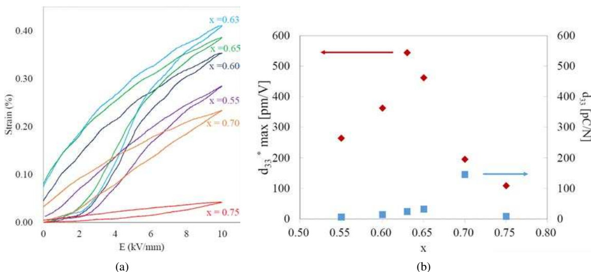
Fig. 26. (a) Unipolar S - E curves; (b) d_{33} and d_{33}^* of unpoled \text{Bi}(\text{Mg}_{2/3}\text{Nb}_{1/3})\text{O}_3 (BMN) doped BF-BT (BT- x BF-BMN, x = 0.55, 0.60, 0.63, 0.65, 0.70 , and 0.75 ) ceramics. 56
