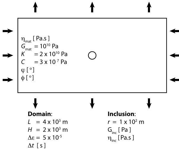
Figure 2. Model configuration and main model parameters. The arrows indicate the pure shear boundary condition which is applied at the model boundaries (incremental displacement). Model parameters that are not defined vary depending to the test case and are listed in Table 1.
