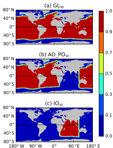
Figure 1. Coupling weights for each coupling region used in the experiments: (a) GL 90 ; (b) AO_PO 90 ; (c) IO 90 . The MC-KPP SST is multiplied by the weight shown and the prescribed SST by (1 - \text{weight}) , and the sum of the two is the boundary condition to the atmospheric grid box. A 10^\circ width (12 grid points) blending is applied at any boundary that is not a coastline. The weights for 200 km and 40 km experiments are the same but with 5- and 30-point blending, respectively.
