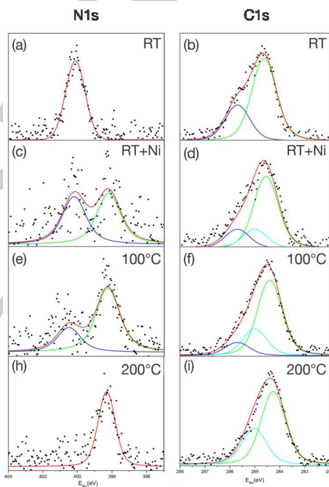
Figure 5. XP spectra of N 1s and C 1s core levels acquired after a) / b) room temperature deposition of HATP on Cu(111), c) / d), after additional deposition of Ni, and annealing to e) / f) 100 °C, and h) / i) 200 °C. Data is represented by black dots; red lines correspond to the sum of all fitted components; N 1s and C 1s components are assigned to the following colour scheme: NH 2 (green), NH-Ni (blue), C-C (green), C-NH 2 (blue), C-NH-Ni (light blue).
