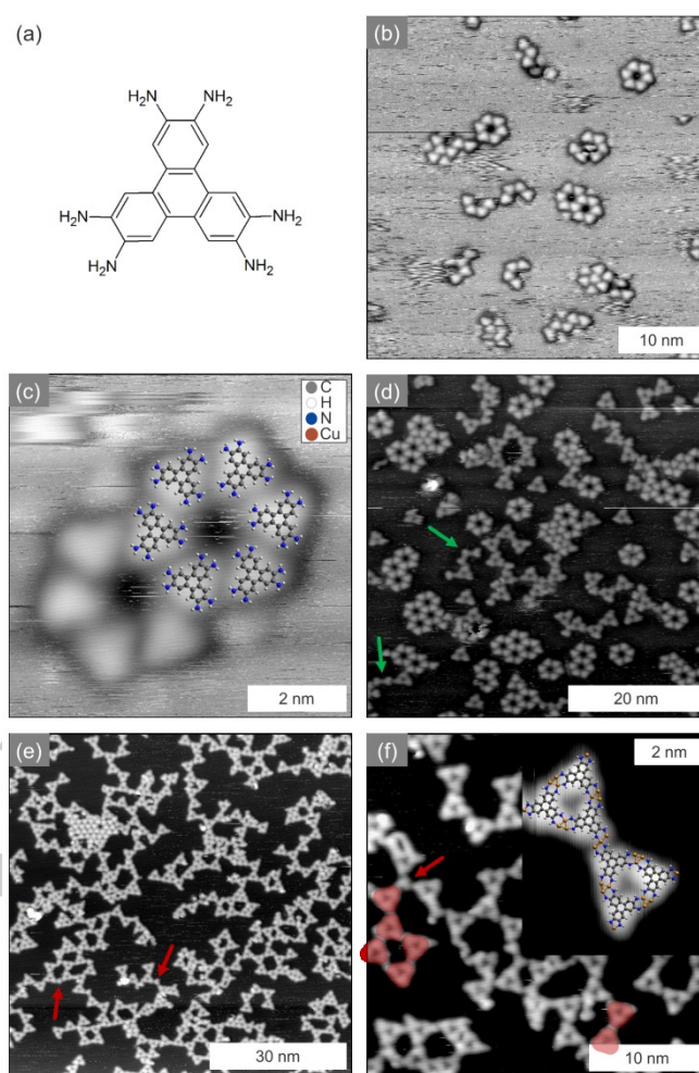
Figure 1. a) chemical structure of HATP; STM images acquired after b) / c) room temperature deposition of HATP onto Cu(111), and after subsequent annealing to d) 100 °C and e) / f) 200 °C; DFT-optimized structures were used for the overlays. c) depicts a HATP decamer comprised of two fused cyclic hexamers; d) annealing to 100 °C results in a mixture of van-der-Waals bonded and metal-coordinated structures; e) overview over predominantly metal coordinated structures obtained after annealing to 200 °C. The close up in f) shows that kinked dimers of Cu 3 -coordinated molecular trimers (examples highlighted in red) represent the most abundant motif. The insert shows a close up of such a kinked dimer overlaid by a structure with a metal-coordination interlink comprised of three copper atoms. Green arrows indicate straight dimers, red arrows highlight single HATP molecules that interlink supramolecular trimers. tunneling parameters: a) 0.73 V, 54 pA; b) 0.73 V, 51 pA; c) 0.89 V, 59 pA; d) 0.87 V, 90 pA; (d, inset) 0.33 V, 20 pA)
