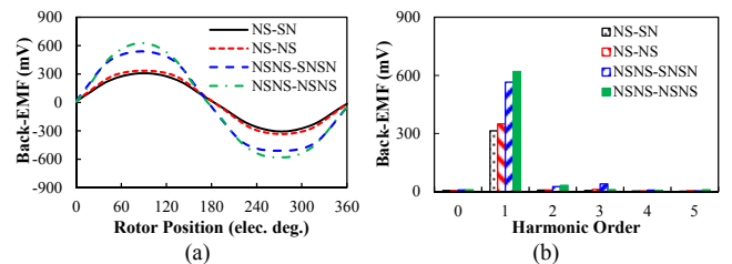
Fig. 17. Phase back-EMF of four FRPM machines ( n=1000 rpm, N_{ph}=4 ). (a) Waveforms. (b) Harmonic spectra.
