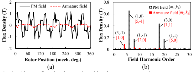
Fig. 3. Air-gap flux density produced by the PM MMF and armature MMF in the NS-SN. (a) Waveforms. (b) Harmonic spectra.
