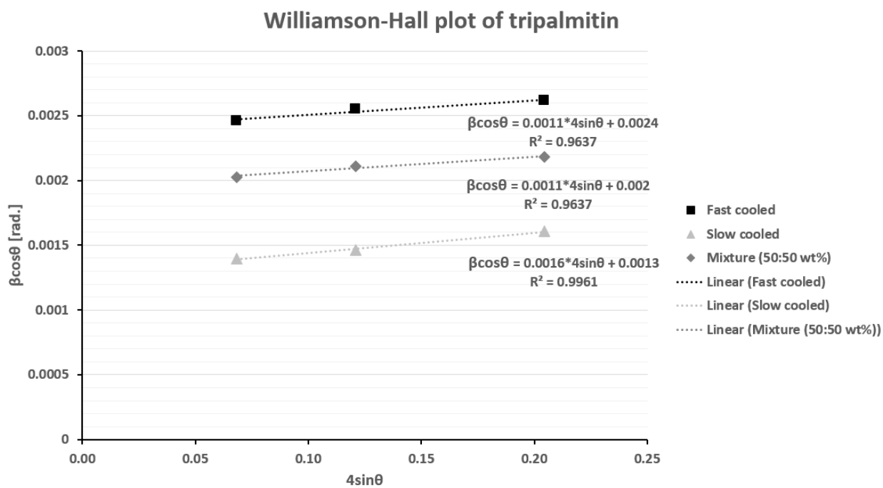
Figure S2. Williamson-Hall plot of long spacing peak broadening of tripalmitin obtained from synchrotron SAXD patterns (Figure S1).
