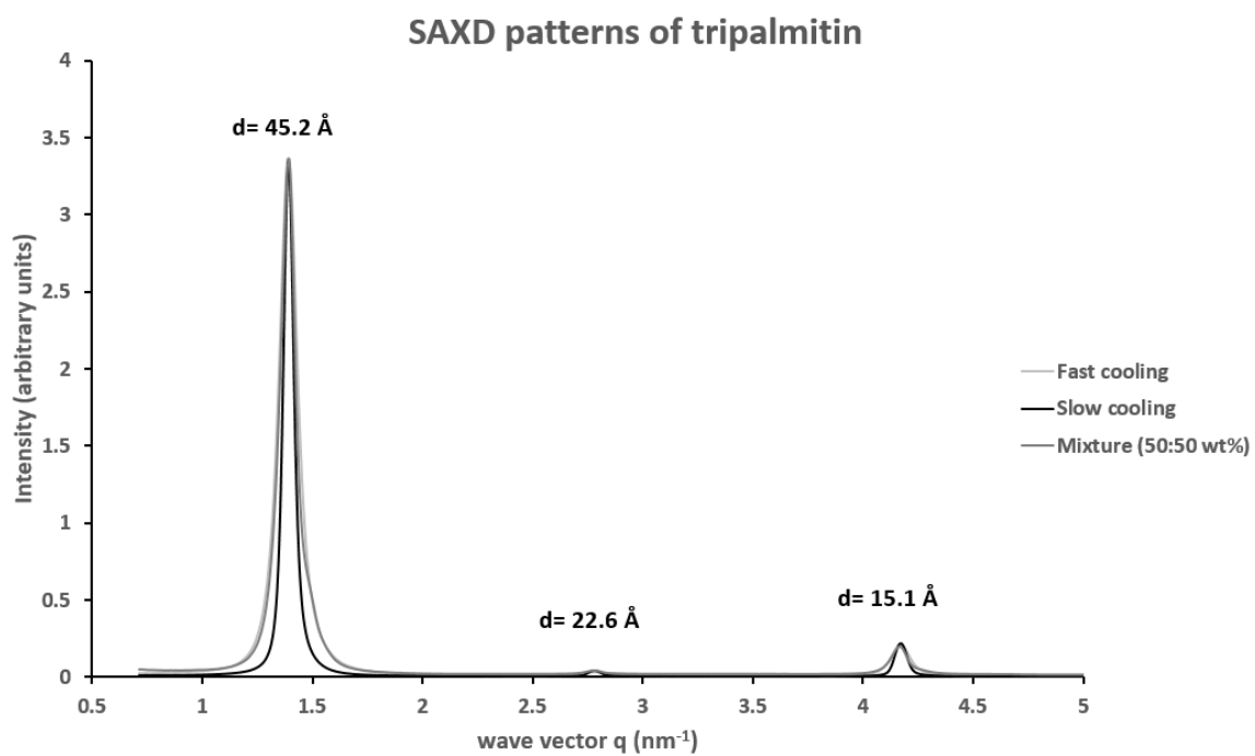
Figure S1. Synchrotron SAXD patterns of tripalmitin crystallized at different thermal conditions.
