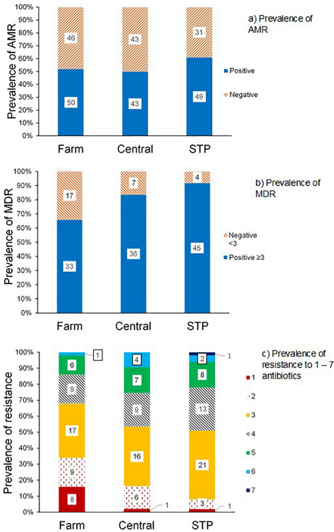
Fig. 3. Site-specific patterns of resistance in E. coli isolates: a) AMR: The percentage of faecal samples which contained E. coli susceptible to ≥1 antimicrobial (negative = orange hatched bars) or resistant to one or more antimicrobial drugs (positive = solid blue bars); b) MDR - the percentage of samples containing E. coli that were resistant to ≥3 antibiotics (positive = resistant = solid blue bars); c) Prevalence of resistance to 1–7 different antibiotics. The sites were Farm, Central and STP.
