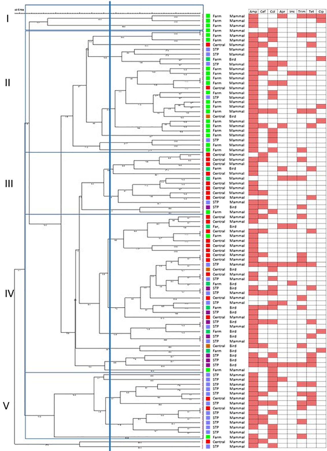
Fig. 2. ERIC profile of E. coli isolated from both small mammals and birds at Farm site (light green, mammals; dark green birds) Central site (red, mammals; dark red, birds) and STP site (light purple, mammals; dark purple, birds). Horizontal lines demonstrate significant clusters (I–V) based on 50% cut-off (vertical line). Red cells demonstrate resistance to each antibiotic: Amp – ampicillin; Cef – cefepodoxime; Col – colistin; Apr – apramycin; Imi – imipenem; Trim – trimethoprim; Tet – tetracycline; Cip – ciprofloxacin.
