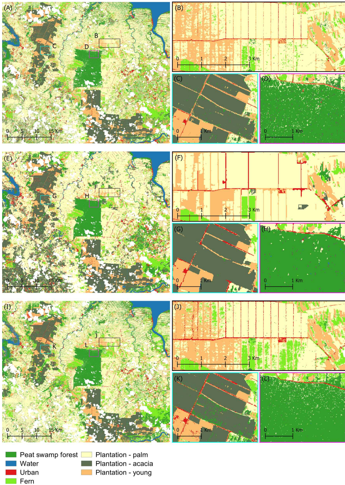
Figure 4. Land cover maps and subsets based on data fusion in the (A–D) pixel-based classification using OPVs, (E–H) object-based classification and (I–L) pixel-based classification using PCs. OPVs, original pixel values; PCs, principal components.
