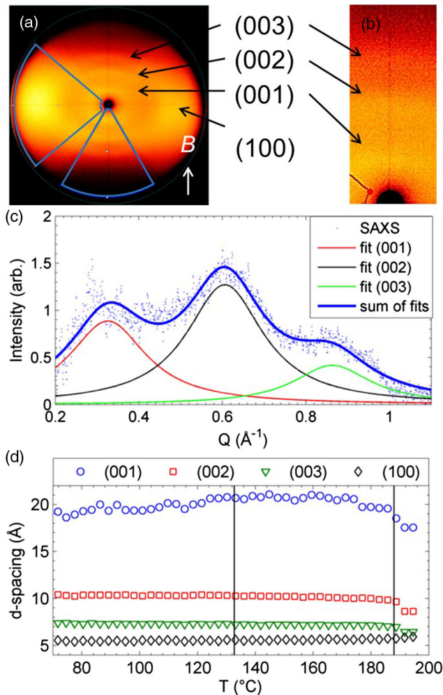
FIG. 9. (a) 2D SAXS pattern of RM734 in the N_S phase at 130°C; the 2D scattering data are radially integrated in the regions defined by the two wedges in (a) to give d-spacings of the (001), (002), and (003) peaks [bottom wedge, see Fig. 9(c)] and the (100) peak (left wedge). (b) Expansion of the small-angle region of (a) showing three weak scattering events. (c) Fitting of raw SAXS data at 80°C to extract d-spacings of the (001), (002), and (003) peaks. (d) Plot of the d-spacings of small- [(001), (002), (003)] and wide-angle [(100)] peaks as a function of temperature. Solid lines correspond to phase transitions.
