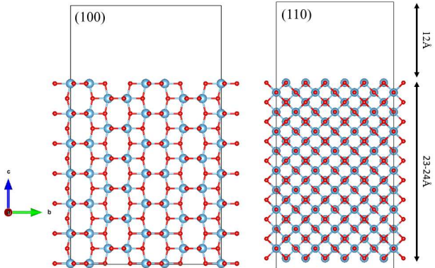
Figure 3: The unit cell of the (100) and (110) surfaces along the a -vector, where the thickness of the vacuum gap and slab thickness are indicated.
