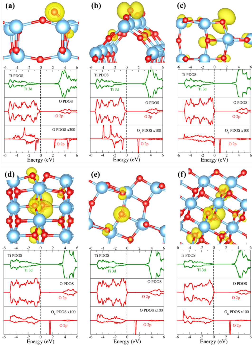
Figure 8: The local geometry (along the a -vector) and PDOS for holes trapped at the (a) 001, (b) 001-recon, (c) 100, (d) 101, (e) 110, and (f) 112, surfaces of anatase TiO 2 . The yellow iso-surface ( 0.0015 \text{ electrons}/a_o^{-3} ) shows the location of the trapped hole polaron, while green and red lines are the Ti 3d and O 2p states, where the dotted black line indicates the position of the Fermi level.
