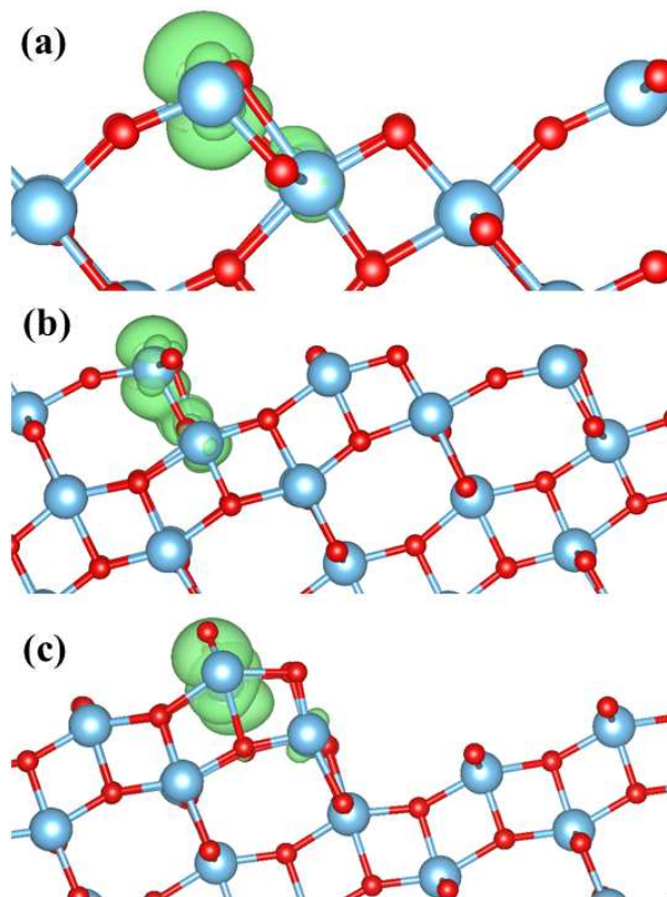
Figure 5: The local geometry (along the a -vector) for electron trapping at the (a) 103, (b) 105 and (c) 107 surfaces of anatase TiO 2 . The green iso-surface ( 0.0015 \text{ electrons}/a_o^{-3} ) shows the location of the trapped electron at the step.
