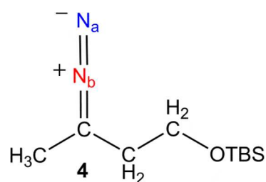
Scheme 5. Structure of the Diazo-Compound 4 Formed by Photoisomerization of the ^{15}\text{N} Labeled Diazirine, 2
