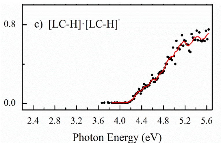
Figure S7: Photofragment action spectrum for [LC-H]·[LC-H] - (m/z = 482) produced from m/z = 241 parent ion.
