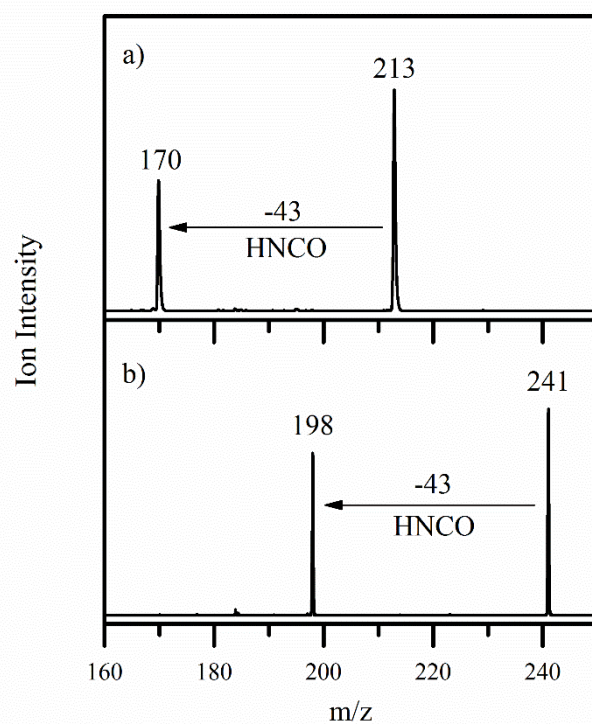
Figure S5: CID mass spectra of a) [\text{AL-H}]^- and b) [\text{LC-H}]^- fragmented with a fragmentation amplitude of 0.47 V for [\text{AL-H}]^- and 0.43 V for [\text{LC-H}]^- . Neutral losses required to produce the photofragments are included.
