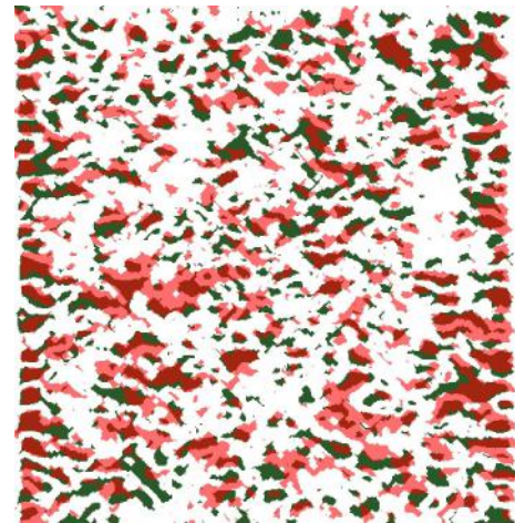
FIG. 4. The 363 K XMCD image from the heating arm (green) and 352 K XMCD image from the cooling arm (light red) made binary using a threshold value and overlaid for comparison (overlap dark red). The full 5 \mu\text{m} island is shown. A high percentage of the domain sites are seen to overlap.
