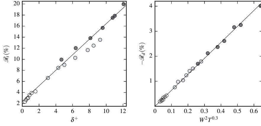
Figure 3: Left: \mathcal{R}_t , the contribution to drag reduction due to the modification to the turbulent Reynolds stresses, versus \delta^+ , the penetration depth of the disc-flow boundary layer. Right: \mathcal{R}_d , contribution to drag reduction due to the disc-flow Reynolds stresses, versus W^2 T^{0.3} . White circles: W^+=3 , light grey: W^+=6 , dark grey: W^+=9 .
