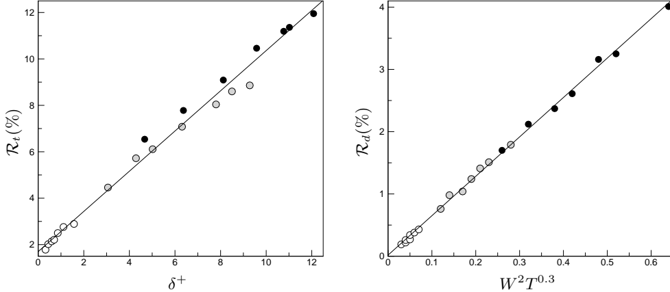
Figure 15: Left: \mathcal{R}_t , the contribution to drag reduction due to turbulent Reynolds stress attenuation, vs. \delta^+ , the penetration depth, defined in (4.5). Right: \mathcal{R}_d , the contribution to drag reduction due to the disc-flow Reynolds stresses, vs. W^2 T^{0.3} . The diameter is D = 6.76 . White circles: W^+ = 3 , light grey: W^+ = 6 , black: W^+ = 9 .
