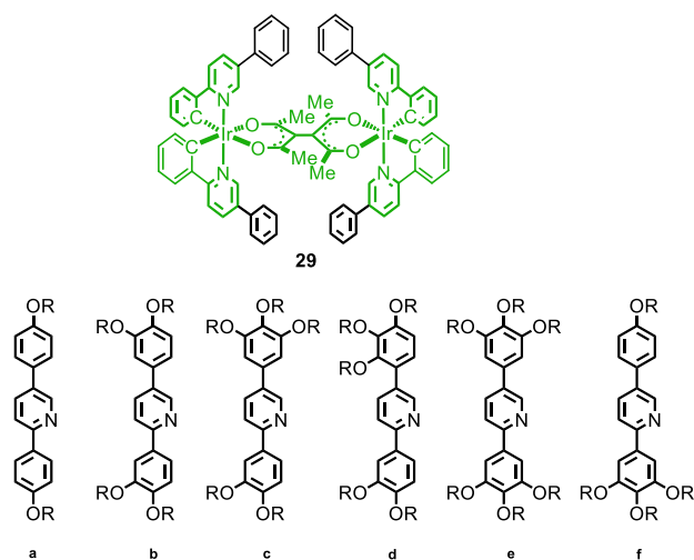
Figure 22 Meso form ( \Delta , \Lambda ) of phosphorescent, liquid-crystalline, dinuclear iridium(III) complexes – peripheral alkoxy chains removed for clarity; 2,5-phenylpyridine ligands used in the study ( R = C_{12}H_{25} ). (Needs copyright permission). Adapted from ref. 89, copyright 2012, Wiley-VCH.
