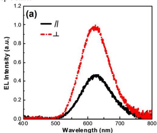
Figure 14. EL spectra of 18a (R = OC n H 2n+1 , n = 6) measured with the polarisation parallel (//) and perpendicular (∞) the rubbing direction. Adapted from ref 74. Copyright 2011, Elsevier Science.
