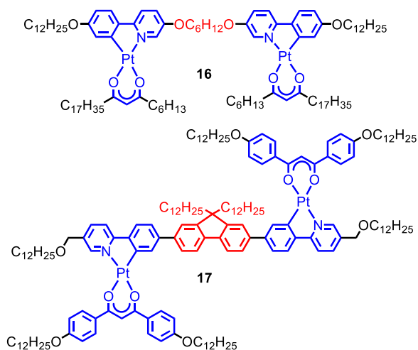
Figure 11. Chemical structures of 16 and 17 . Adapted from ref. 60 ( 16 ), copyright 2015, Elsevier Science. Adapted from ref. 61 ( 17 ), copyright 2012, American Chemical Society.
