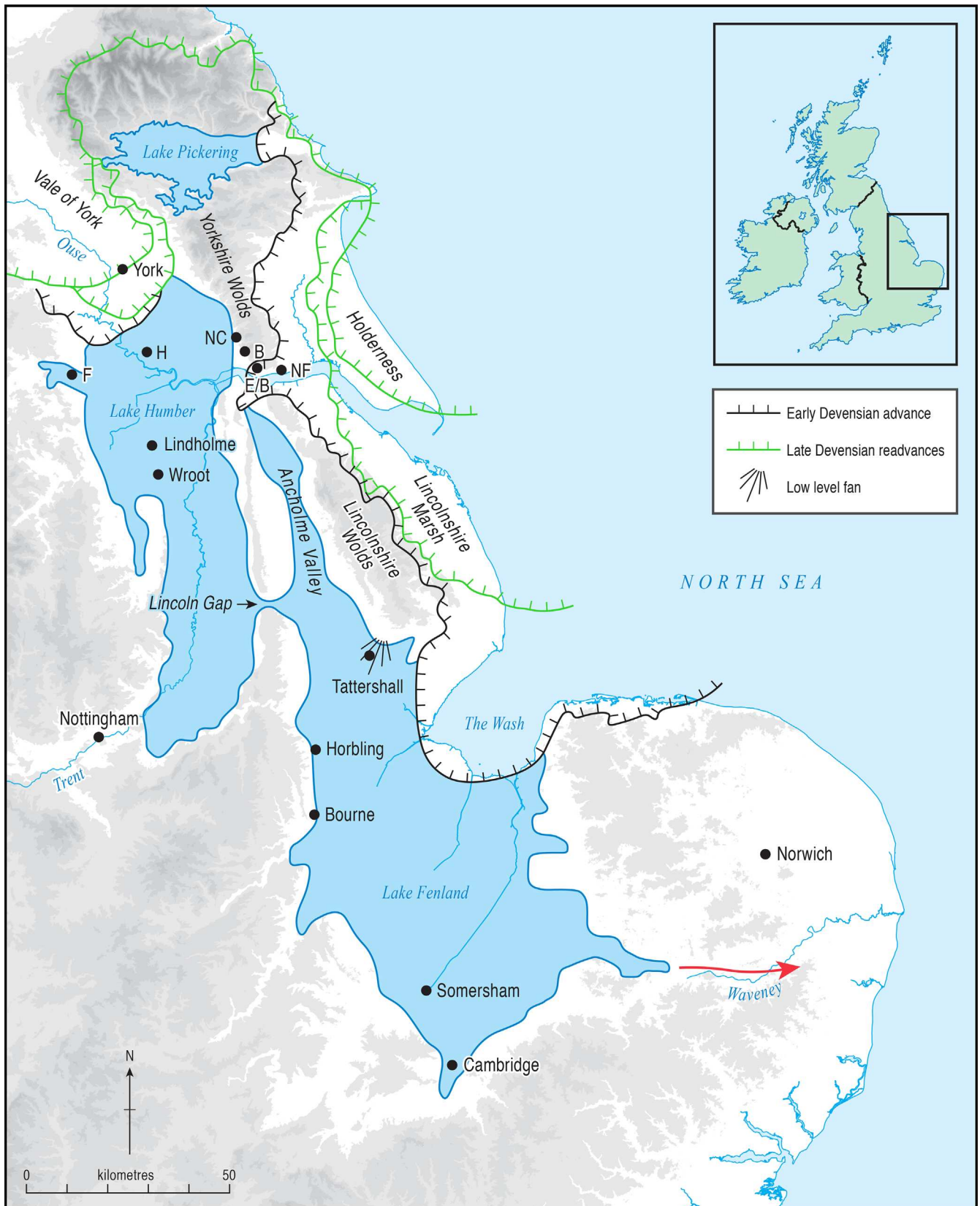
Figure 1. The proposed extents of Devensian glaciation and the glacial Lake Humber/Fenland high-level (ca. 30 m OD) phase during the early Devensian (MIS 4) as proposed by Straw (1979). Red arrow represents the proposed spillway along the Waveney valley. The 'low level fan' at Tattershall is incised into the MIS 6 Kirkby Moor Sands and emerges from the mouth of the lower Bain valley, Lincolnshire. Contours are shown at 50 and 100 m, and at 100-m intervals thereafter. Adapted from Straw (1979) and Murton and Murton (2012). Locations cited in the text are: B – Brantingham; E/B – Elloughton/Brough; F – Ferrybridge; H – Hemingbrough; NC – North Cave; NF – North Ferriby.
