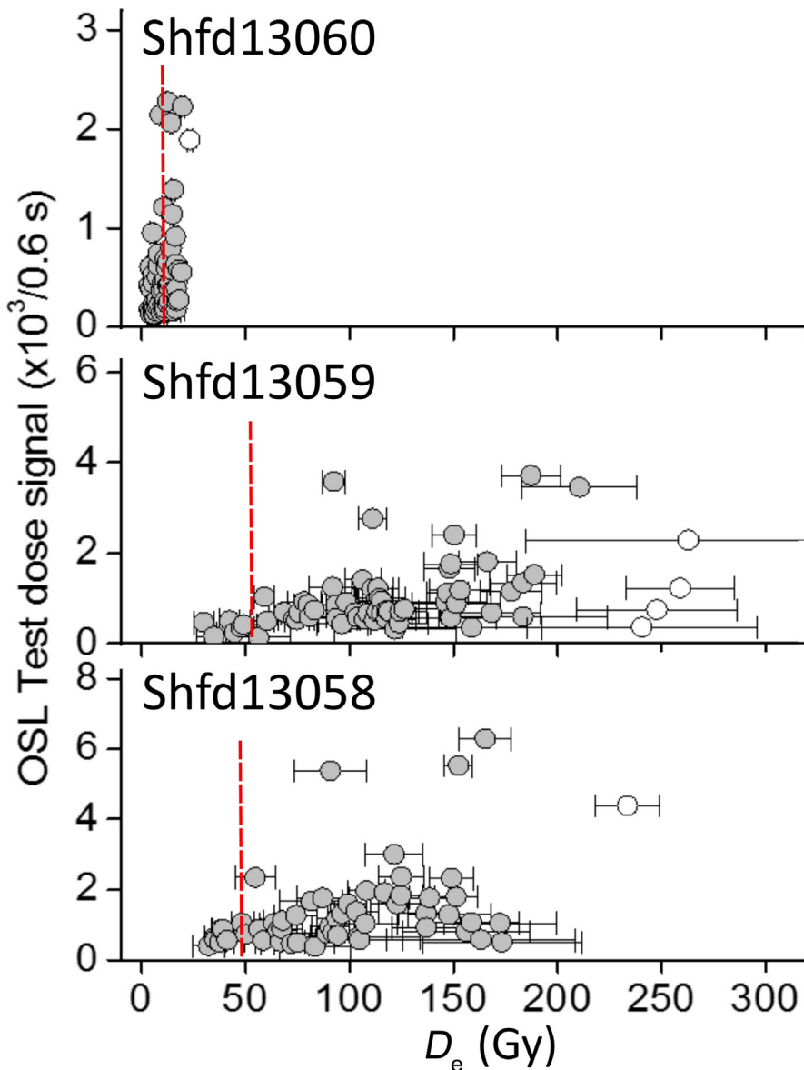
Figure 10. D_e distributions from the three samples. Plots show the OSL natural test dose response as a function of D_e . Each point corresponds to the measurement of an individual multi-grain aliquot. Identified outliers are shown as open circles in the plots. The red dashed line indicates the D_e used for age calculation purposes.
