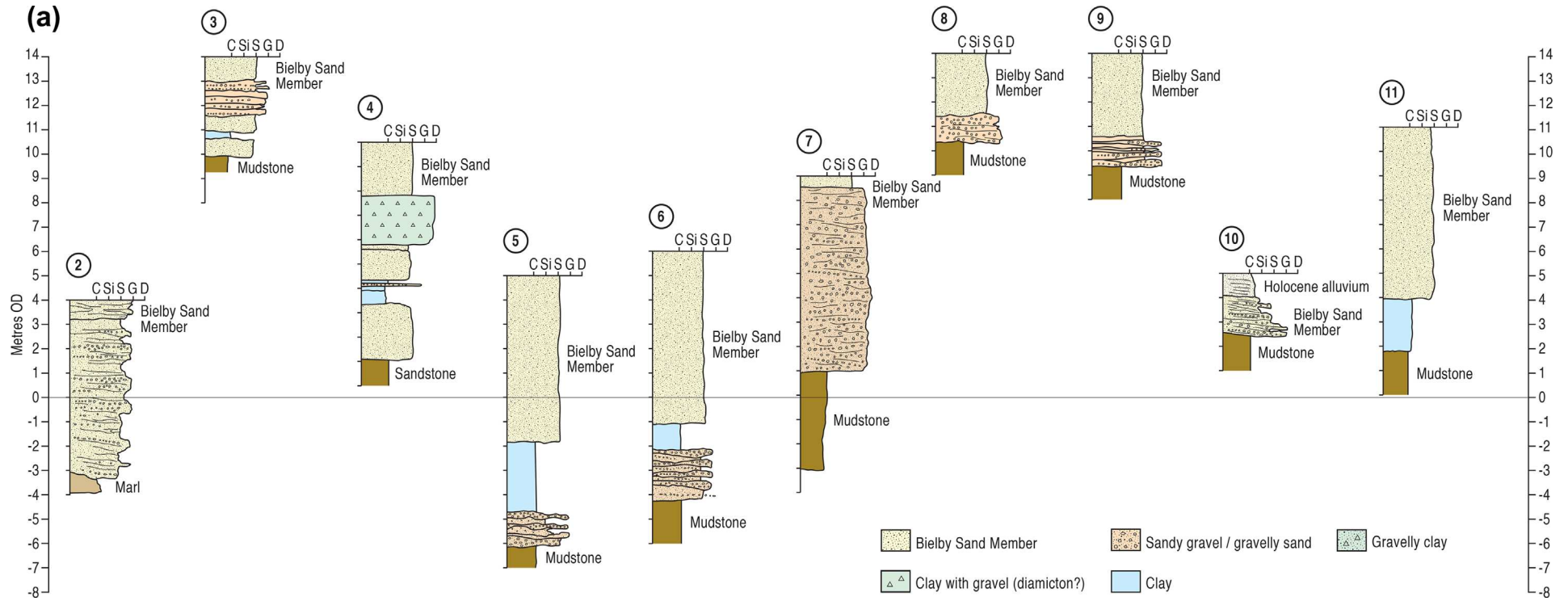
Figure 9. Borehole logs extracted from the BGS borehole data archive and located on Fig. 2C (except site 4 which is near Brough on Fig. 2A): (a) individual logs from around the study area; (b) logs from intensively sampled site at Sand Lane, immediately south-east of North Cave and arranged along two transects as identified in Fig. 2 by the label SL; (c) correlation of stratigraphic units along a transect from the Wolds scarp slope to the head of the Humber Estuary using selected borehole logs, BGS mapping and employing the formation and member nomenclature of the BGS.
