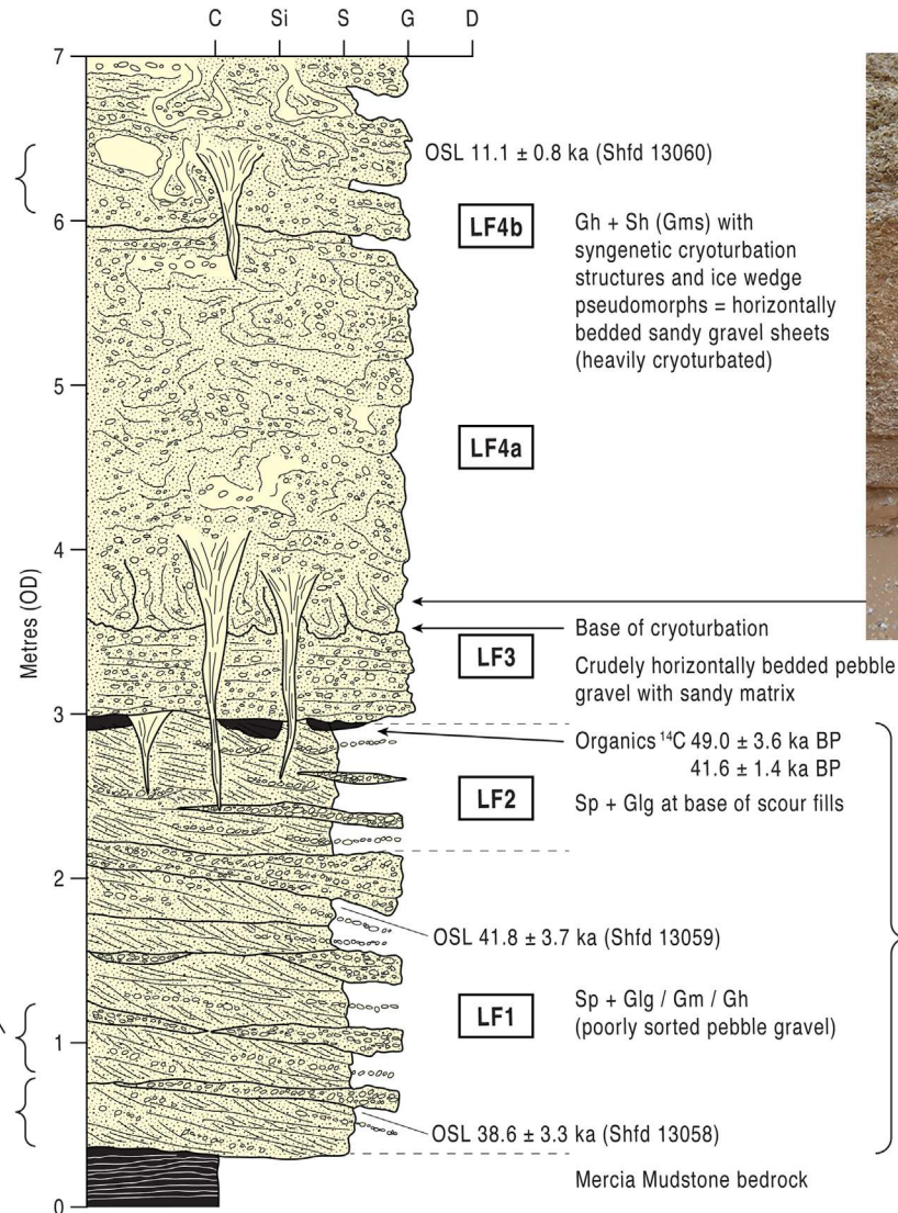
Figure 4. Composite vertical profile log (a) and clast lithologies for selected facies (b) from the exposure at North Cave. The log shows major lithofacies and the internal structures, clast form and palaeocurrent data (based on downflow dip directions of avalanche or lee side beds in cross-bedded sands), and locations of OSL and ^{14}\text{C} dates. Inset photograph shows the nature of syngenetic ice wedge pseudomorphs developed in the base of LF4a and extending down into LF3 and LF2.
