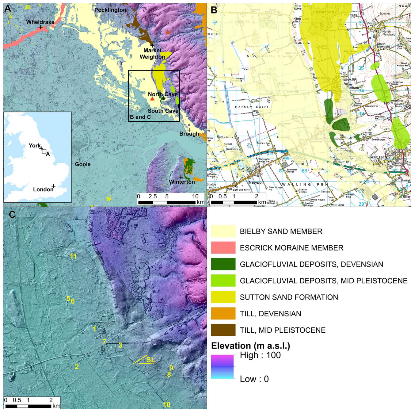
Figure 2. Location maps (derived from Digimap) showing (A) the distribution of the main surficial geology units and LiDAR images for the south-east corner of the Vale of York and adjacent Humber lowlands and Yorkshire Wolds. (B) Enlargement of geological units in the study area. (C) LiDAR and borehole log locations (marked in yellow) and North Cave quarry (red triangle) in the study area.
