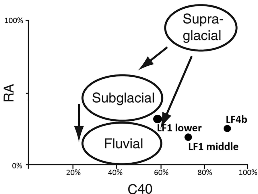
Figure 8. Covariance plot for RA/C40 containing envelopes for samples of known transport origins where clast lithology strongly controls the C40 index to produce abnormally high slabiness/platiness (from the Type II plot of Lukas et al. , 2013).
