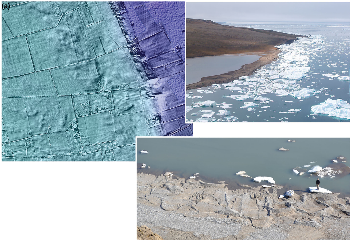
Figure 11. Landforms on the southern Vale of York/Humber lowlands and probable modern analogues: (a) LiDAR image showing overprinted hummocky and arcuate ridges at the Wolds scarp footslope and examples of the most likely modern analogues of floating ice push ridges on the coast of Banks Island, Arctic Canada; (b) LiDAR image showing, at the top, discontinuous sinuous ridges connecting with oval to circular rimmed depressions and, at the base, dual ridged polygonal forms. Examples of modern analogues from recently drained, aggrading permafrost terrains in Arctic Canada are depicted at right, with the upper images showing ice wedge and pingo complexes from Banks Island, and the lower images showing ice wedge landforms from northern Ellesmere Island.
