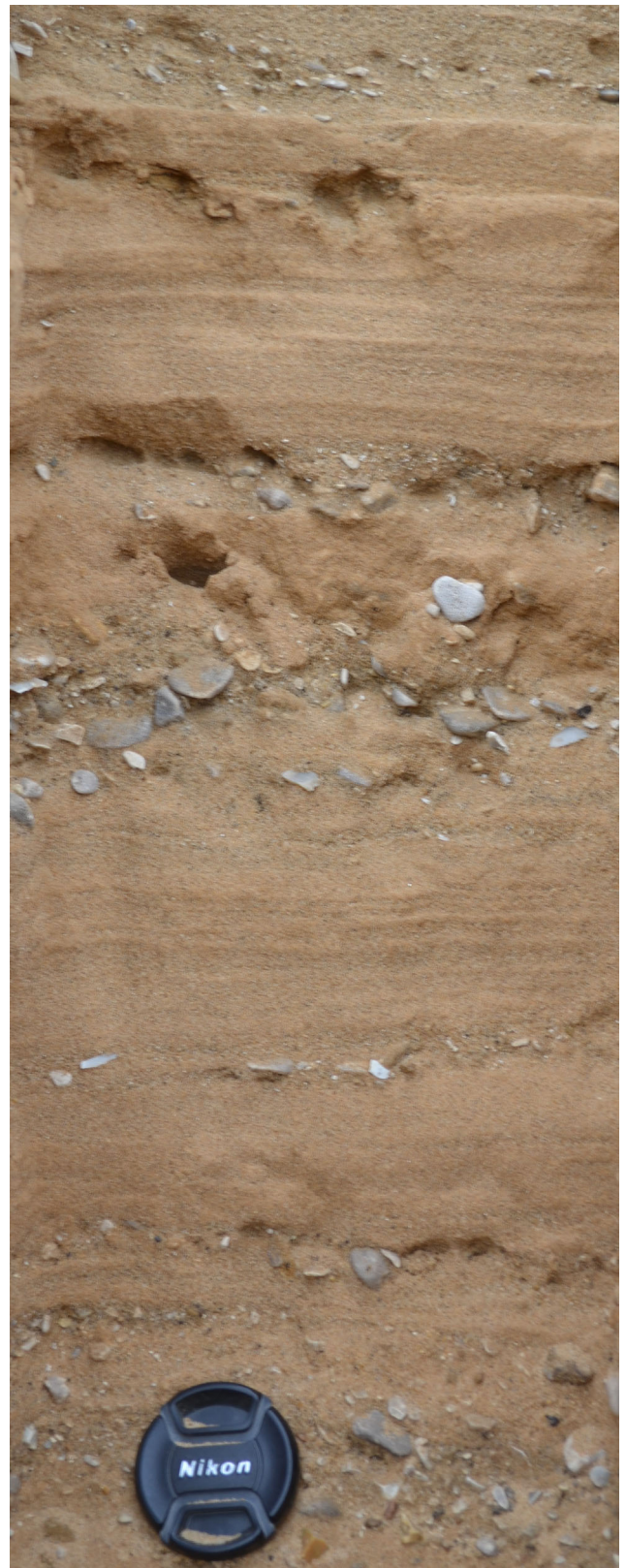
Figure 5. Details of LF1, showing horizontal to low angle planar cross-bedded sand with lags, separated by discontinuous lenses to beds of massive to horizontally bedded gravel.
