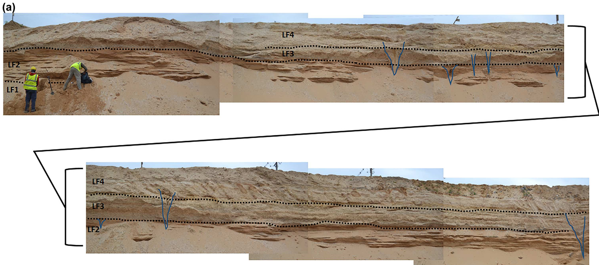
Figure 3. Details of the North Cave stratigraphy. (a) Photomosaic of the main quarry face at North Cave, showing the tabular nature of the lithofacies and the distribution of secondary, vertically aligned structures (ice wedge pseudomorphs) in blue (b) Variety of well-developed periglacial and permafrost features, including: A – simple ice wedge pseudomorph developed in gravels and extending down into sands and sandy gravels in which an earlier ice wedge appears to have been developed, thereby constituting an interformational structure; B – simple ice wedge pseudomorph in gravel extending down to a sand wedge in underlying sandy facies; C – composite wedge pseudomorph extending downwards from LF4a and cross-cutting LFs 3 and 2. Such wedges comprise a primary infill pipe at the centre, here composed of a sand wedge, and a secondary outer zone of normal faults in the host gravel related to secondary infilling in association with the ice wedge; D – multi-layered pendant or tear drop structures/cells of finer-grained sediment and upward penetrating gravel-cored diapirs; E – cryoturbation feature, showing downward loading of gravels and vertical displacement of sandy gravels to form a flame structure.
