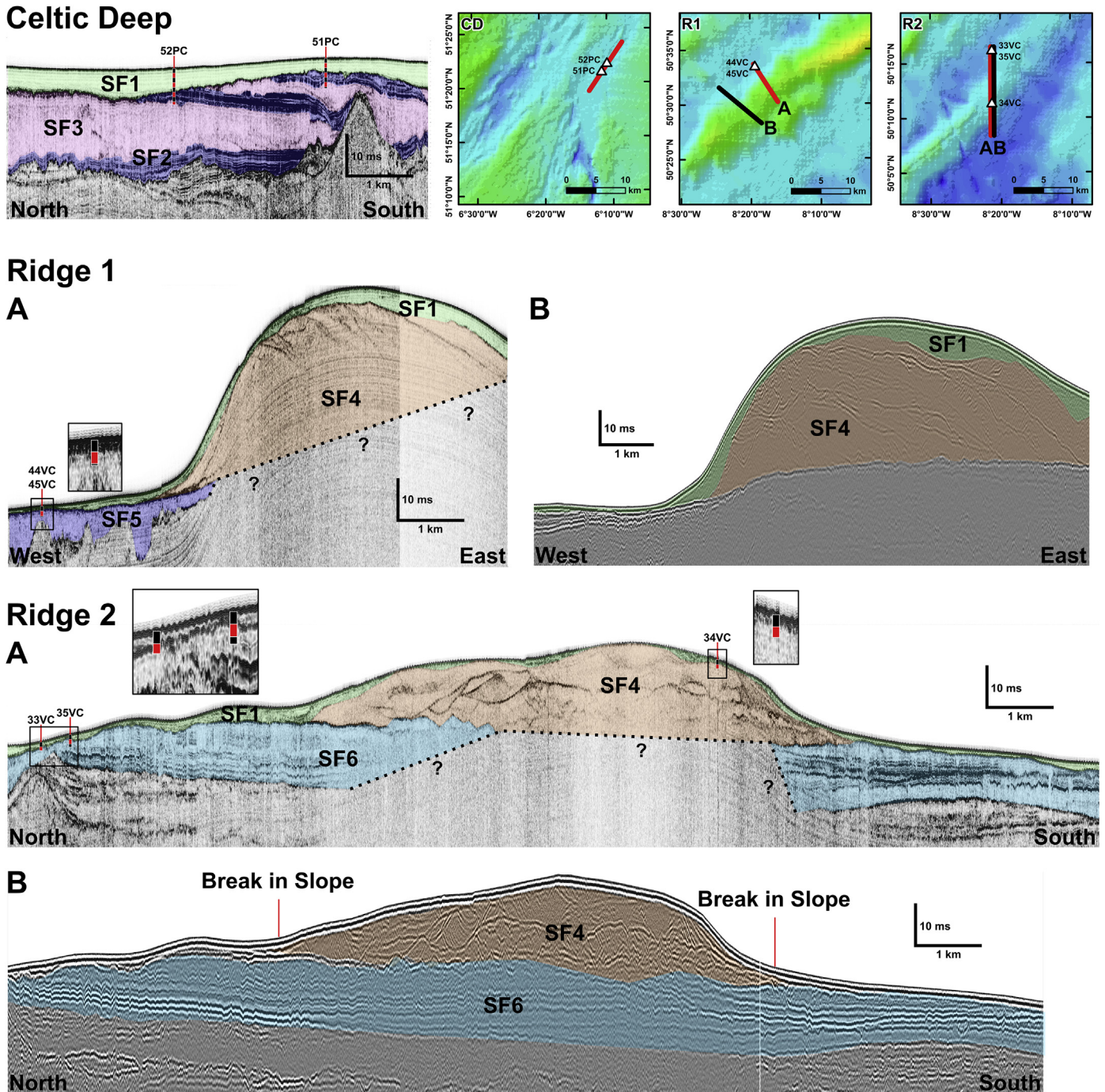
Fig. 3. Seismic-facies of the Celtic Deep based on chirp data, and Ridge 1 and Ridge 2 from chirp (A) and sparker (B) data along the same transects for each megaridge. See Fig. 1 for line and inset locations.
