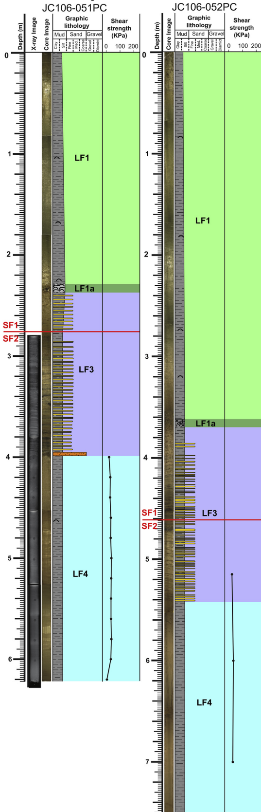
Fig. 2. Lithostratigraphic logs of sediment cores with approximate reflector depths, where resolvable, shown in red using an assumed velocity of 1600 m s -1 . See Fig. 1 for core locations.
