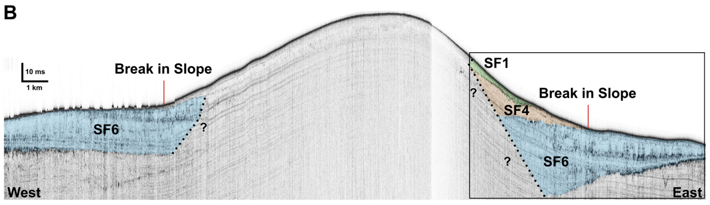
Fig. 5. Seismic-facies based on chirp (A) and sparker (B) data of Ridge 4 and chirp data of Ridge 5 on the eastern flank (A) and across its entire width (B). See Fig. 1 for line and inset locations.
