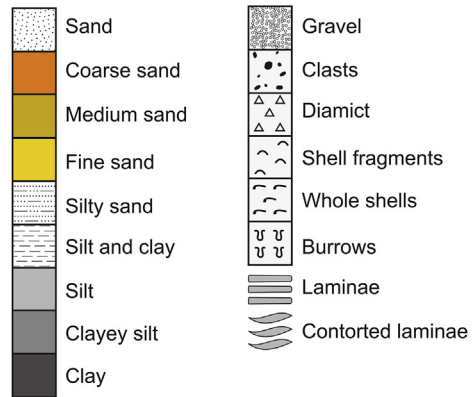
Fig. 2. Lithostratigraphic logs of sediment cores with approximate reflector depths, where resolvable, shown in red using an assumed velocity of 1600 m s -1 . See Fig. 1 for core locations.
