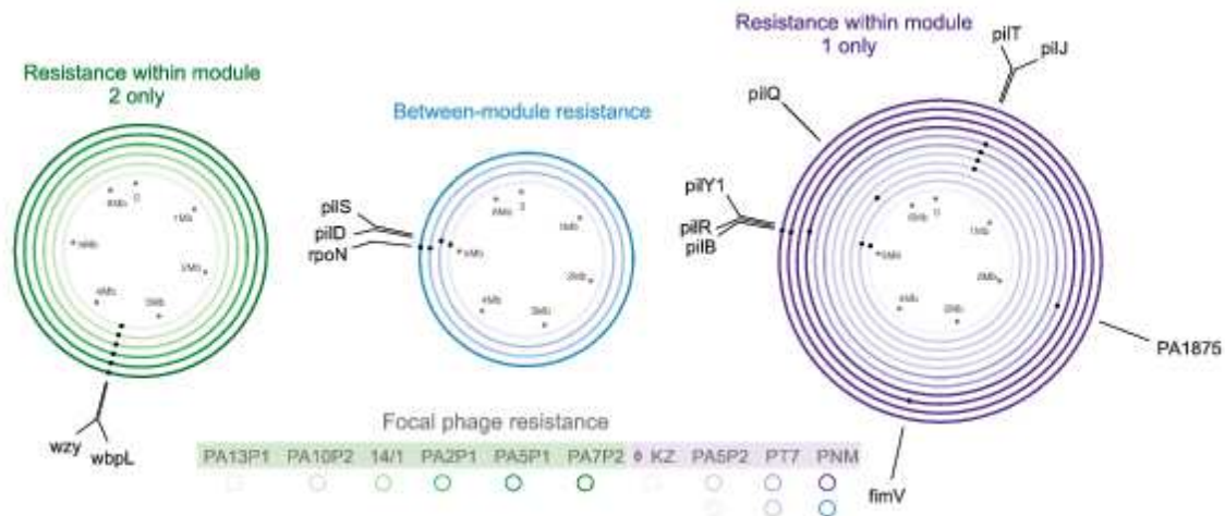
Fig 3. Genetic basis of phage resistance
