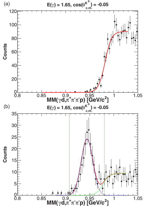
FIG. 7. The top panel is a hyperbolic tangent curve fit to the missing mass of \gamma d \rightarrow K_S^0 \Sigma^0 p \rightarrow K_S^0 \Lambda(\gamma p) \rightarrow \pi^- \pi^+ \pi^- p(\gamma p) from simulation. The bottom panel is a fit to the missing mass of an example data bin. The fit uses a Gaussian and a hyperbolic tangent shape that was parametrized from the simulation. This is an example of the g13 data fit to extract the number of events that were missing only one proton.
