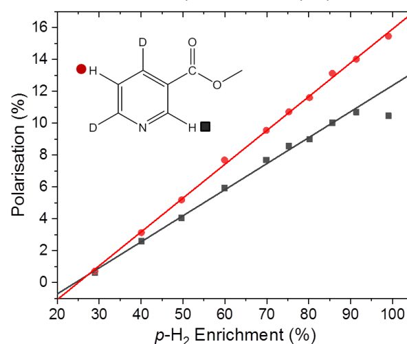
Figure 5. Methyl-4,6- d 2 -nicotinate hyperpolarisation level under SABRE as a function of p -H 2 enrichment. Spectra were acquired on a 1 T benchtop NMR spectrometer (Magritek Spinsolve Carbon) and used the [IrCl(COD)](IMes) pre-catalyst in methanol- d 4 . The final point at 99% p -H 2 enrichment was acquired using a 30° pulse for both the SABRE experiment and corresponding thermal reference. The H2 ( ortho ) position proton resonance still retained some antiphase character and gives a slightly reduced overall polarisation level as a consequence; it is omitted from the linear fit.
