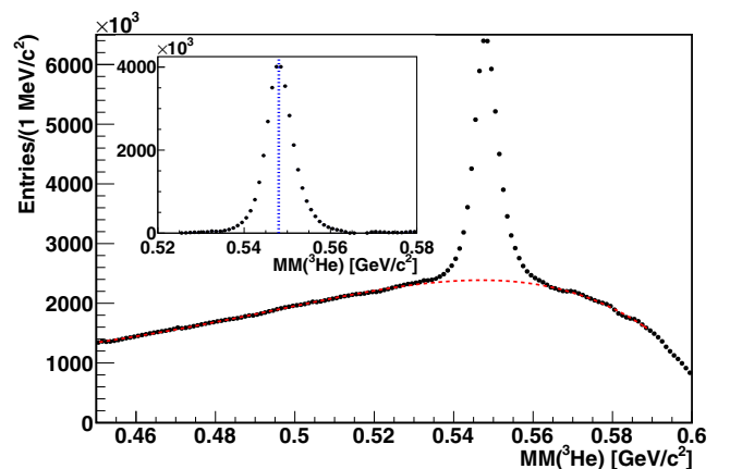
FIG. 2. Initial spectrum of the {}^3\text{He} missing mass. The prominent peak is due to \eta meson production, while the broad background distribution is from production of two and three \pi mesons. The dashed (red) line shows a fit of the background (incorporating the shapes of double and triple \pi meson production, as described in the text) and the inset shows the peak after background subtraction with the \eta mass marked by the dotted (blue) line.
