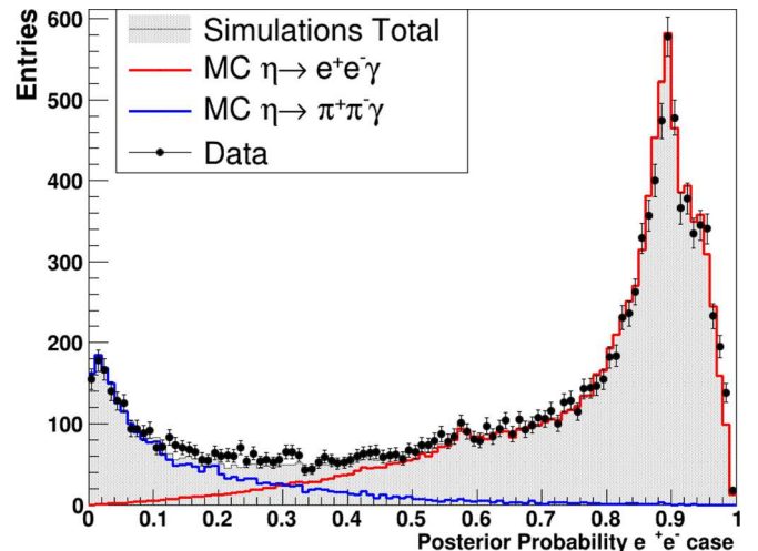
FIG. 6. Posterior probabilities for events passing the \eta \rightarrow e^+e^-\gamma kinematic fit hypothesis showing the discrimination of \pi mesons from electrons. The red and blue lines are simulations of \eta \rightarrow e^+e^-\gamma and \eta \rightarrow \pi^+\pi^-\gamma respectively and the shaded area is the sum of both simulations.
