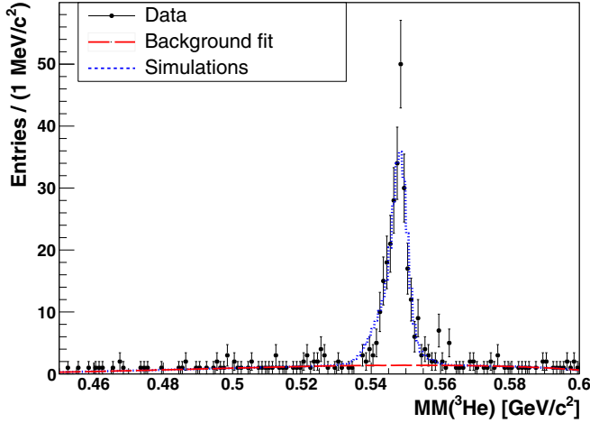
FIG. 15. The MM(^3\text{He}) distribution for events passing the \eta \rightarrow \pi^+\pi^-e^+e^- selection criteria. The background fit is shown as a dashed line (red) and the shape of the peak from simulations of the pd \rightarrow ^3\text{He} \eta events is shown as a dotted line (blue).
