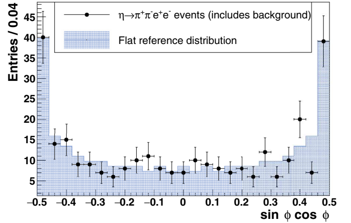
FIG. 16. \sin \phi \cos \phi distribution for the data and Monte Carlo simulation of the \eta \rightarrow \pi^+\pi^-e^+e^- with a flat \phi distribution.
