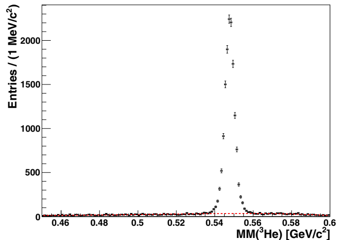
FIG. 9. {}^3\text{He} missing mass distribution for events passing all selection conditions for \eta \rightarrow e^+e^-\gamma . The background fit is described by the dashed line.
