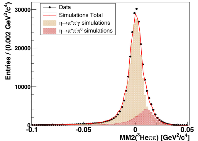
FIG. 12. The experimental MM^2(^3\text{He} \pi^+\pi^-) distribution for the pd \rightarrow ^3\text{He} \eta events after the kinematic fit probability cut for the pd \rightarrow ^3\text{He} \pi^+\pi^-\gamma hypothesis (points) compared to MC of the \eta \rightarrow \pi^+\pi^-\gamma (light shaded) signal and the \eta \rightarrow \pi^+\pi^-\pi^0 background (dark shaded). The red curve is the sum of the simulations. Kinematic variables used to obtain the distributions are not corrected by the kinematic fit.
