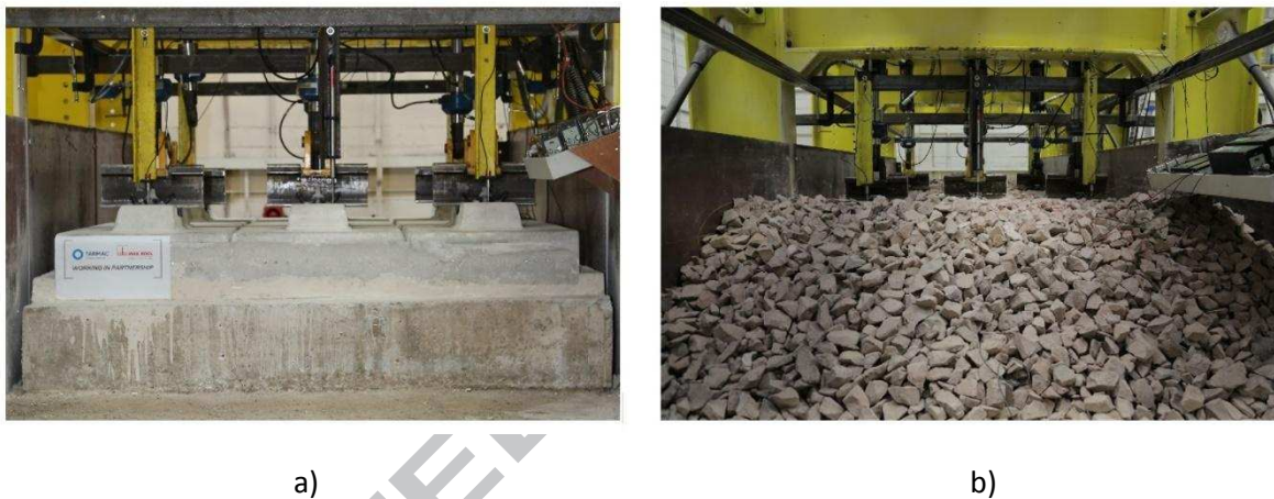
Figure 1: a) Slab track test and b) Ballasted track test in GRAFT-2 facility.
