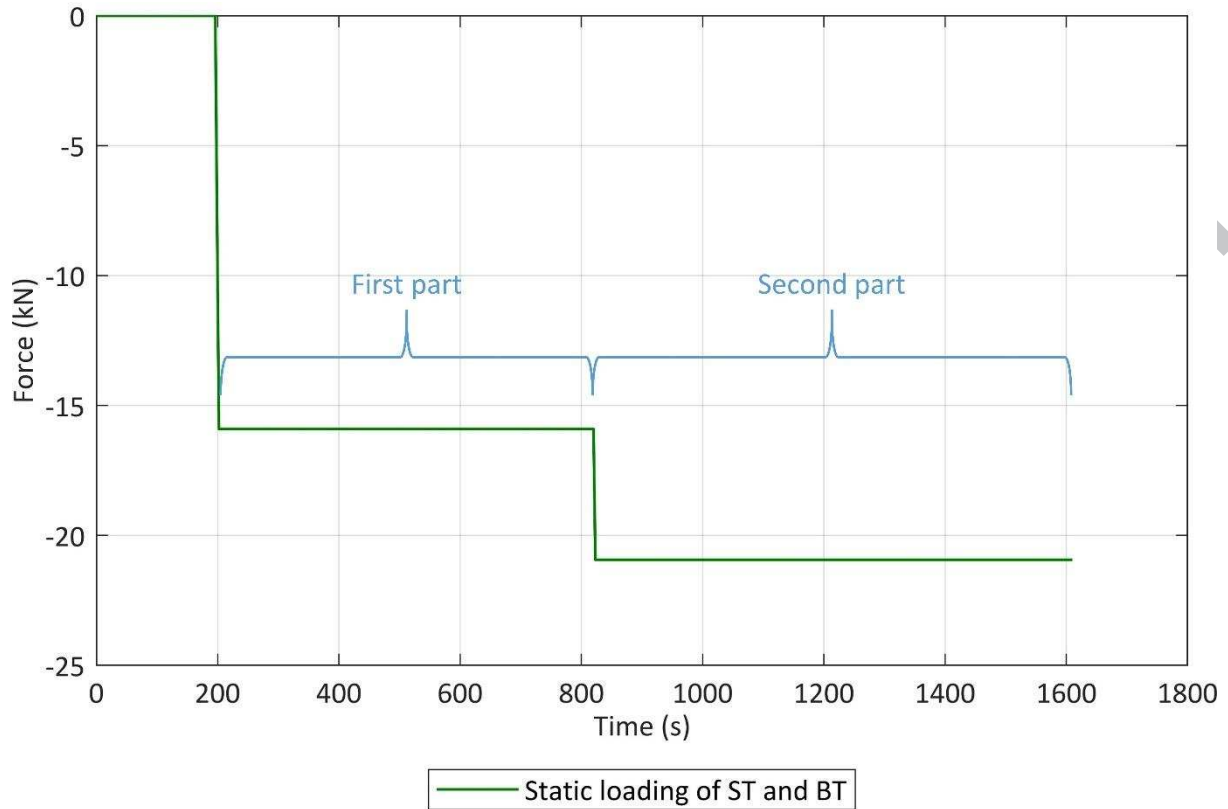
Figure 9: Force vs time for ballasted and concrete slab track.
