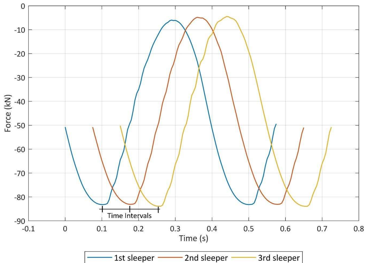
Figure 8: Time interval of sequential loading in one cycle.
