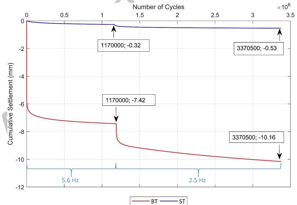
Figure 14: Cumulative settlement of concrete slab track (ST) and ballasted track (BT) vs number of cycles.
