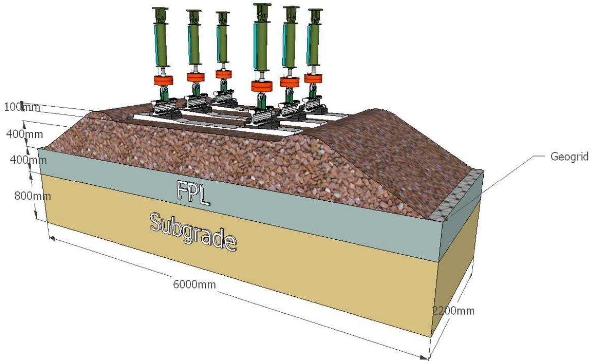
Figure 7: Layout of ballasted track and substructure
