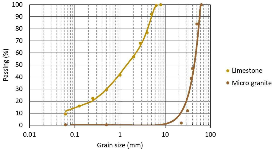
Figure 3: Sieve analysis for limestone and micro granite.
