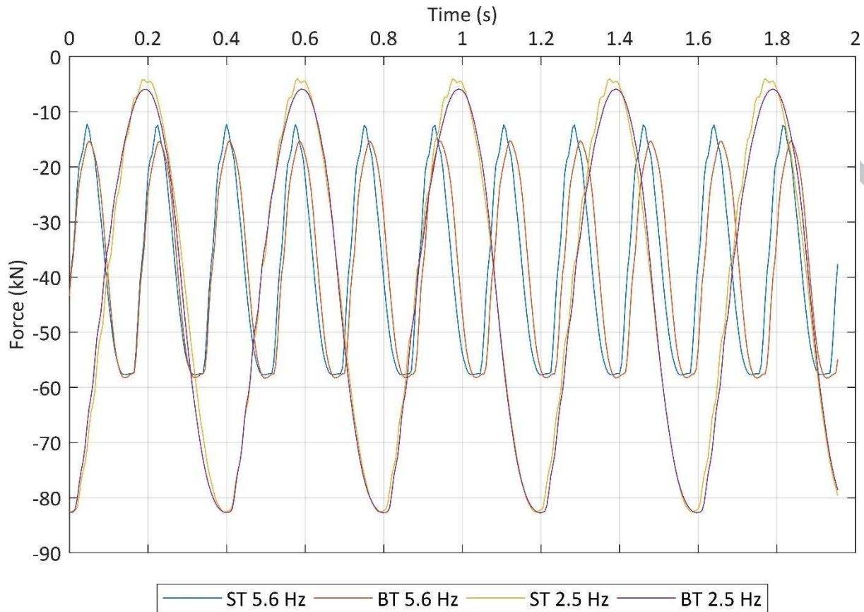
Figure 13: Force vs time for ballasted track (BT) and concrete slab track (ST) at 2.5 Hz and 5.6 Hz.
