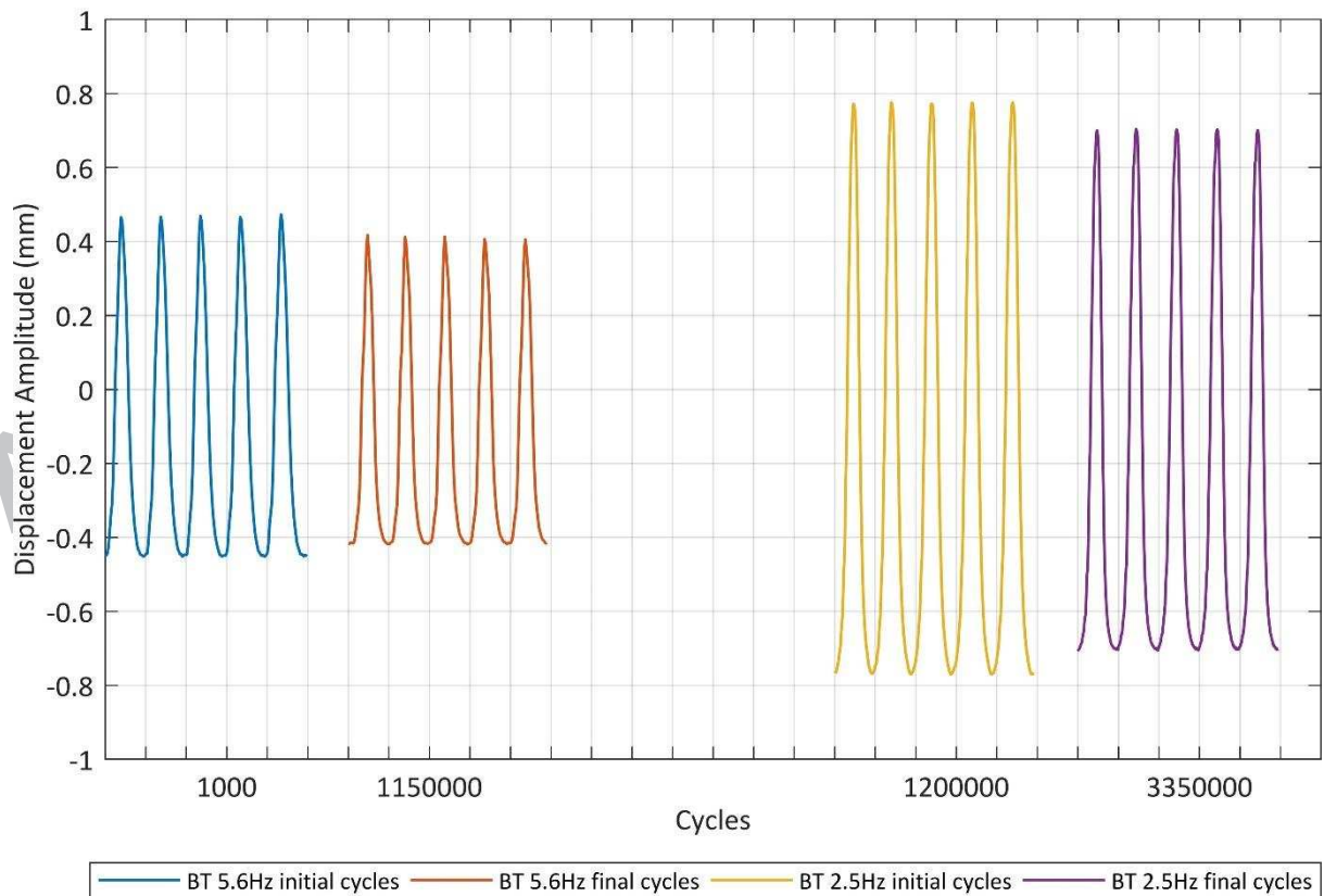
Figure 15: Amplitude of concrete slab track at the beginning and at the end of the 5.6 Hz and 2.5 Hz cycles, respectively.
