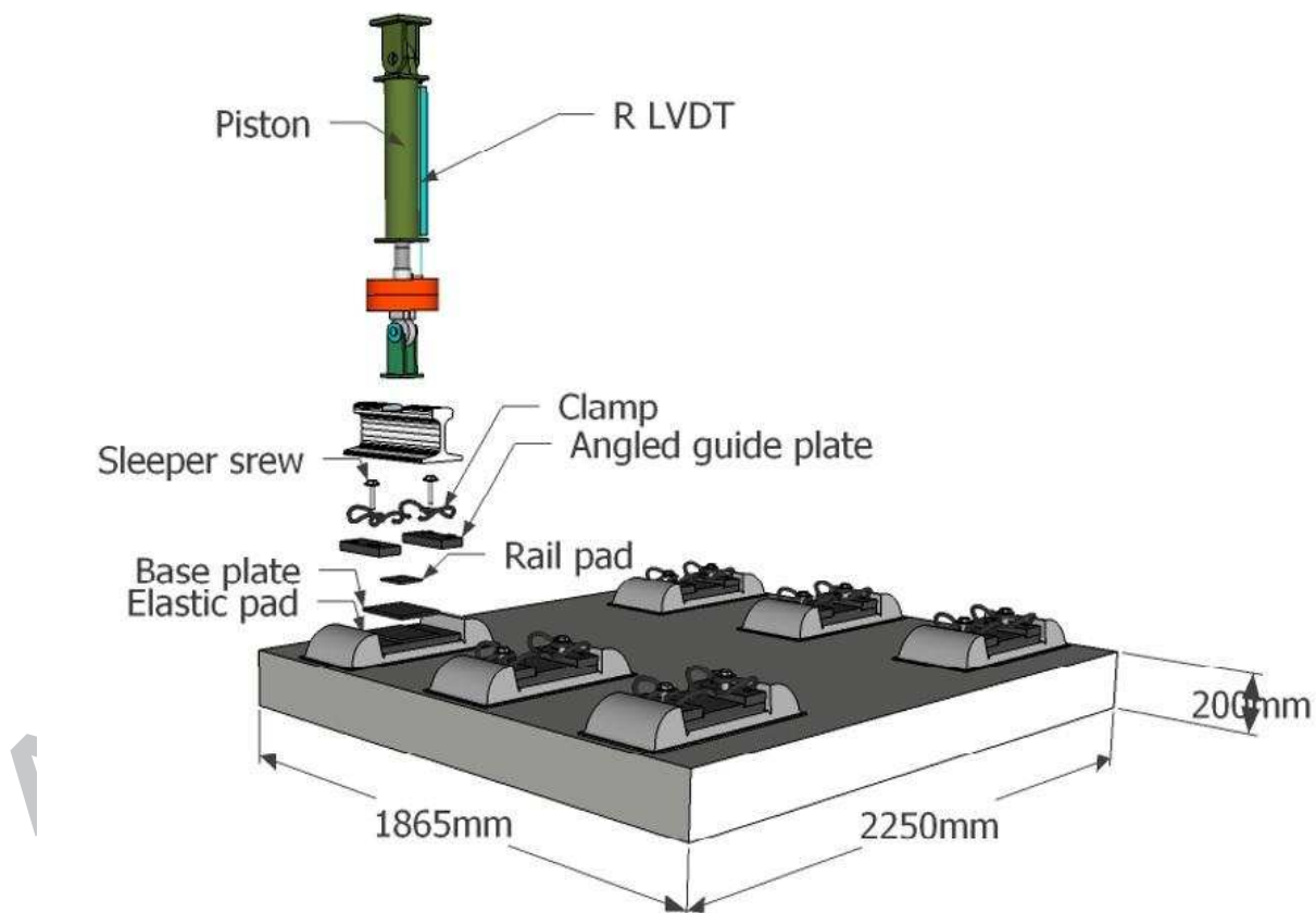
Figure 5: Tack system and loading configuration.
