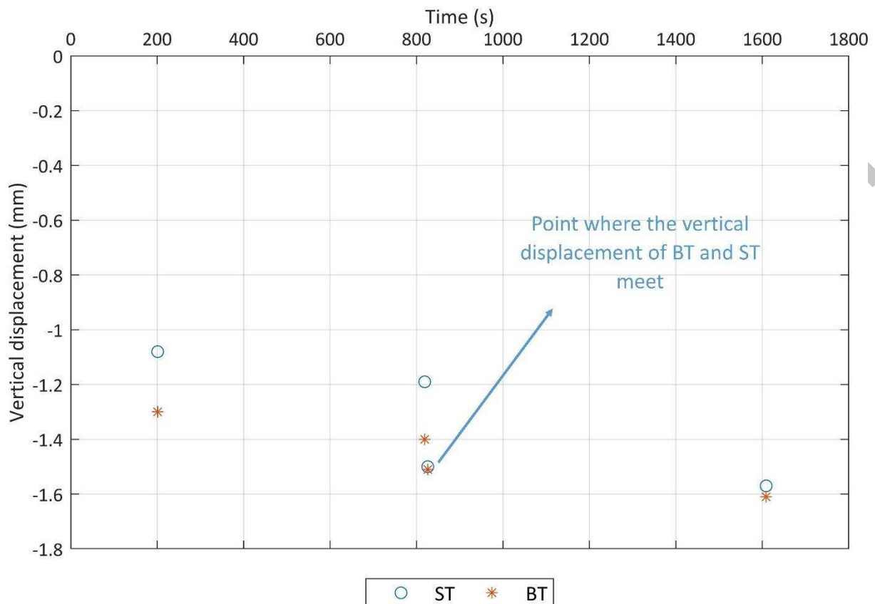
Figure 12: Vertical displacement on the surface of rail for ballasted track (BT) and for slab track (ST) without displacements in the ballast and subgrade, respectively.
