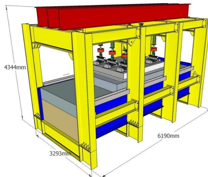
Figure 2: Dimensions of GRAFT-2 facility.
