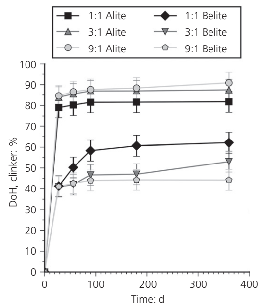
Figure 8. Degree of reaction of calcium silicate clinker phases (alite and belite) within the different blend ratios, based on 29 Si MAS NMR spectral deconvolutions
