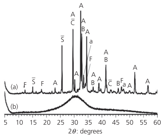
Figure 1. X-ray diffractograms of anhydrous: (a) PC; (b) BFS (A, alite; B, belite; F, ferrite; a, aluminat; C-bar, calcite; S-bar, gypsum)
