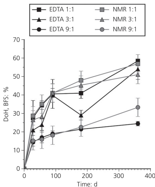
Figure 7. Degree of reaction of BFS within the different blend ratios, based on 29 Si NMR MAS deconvolutions (NMR) and on selective dissolution (EDTA)
