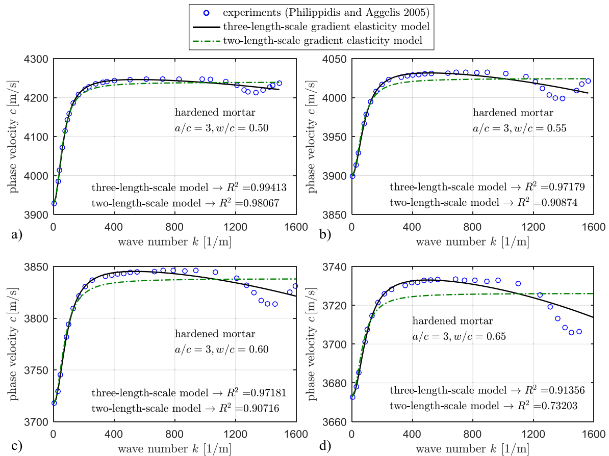
Fig. 8. Analytical versus experimental dispersion curves of hardened mortar specimens with a/c=3 and different w/c ratios: a) w/c=0.50 ; b) w/c=0.55 ; c) w/c=0.60 ; d) w/c=0.65 (experimental data after Philippidis and Aggelis, 2005).
