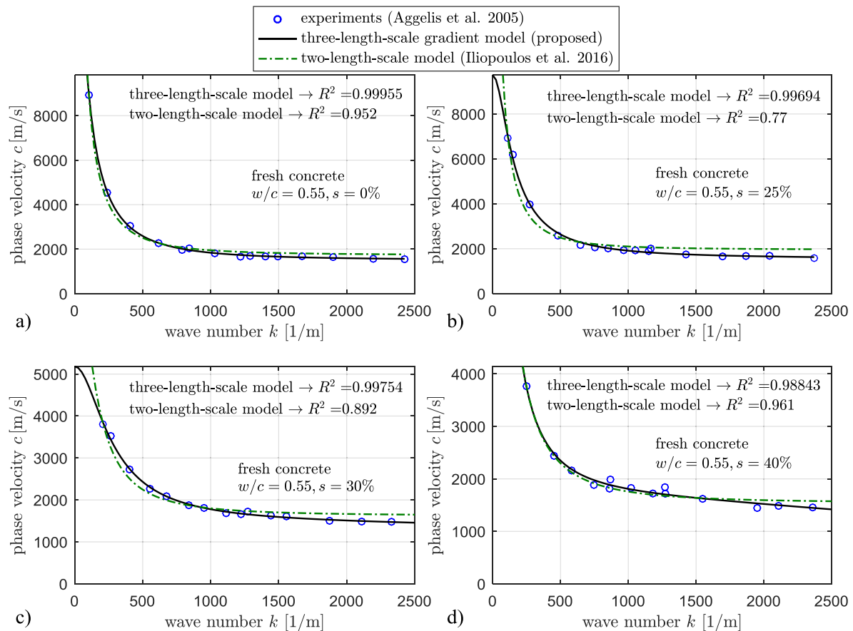
Fig. 6. Analytical versus experimental dispersion curves of fresh concrete specimens with w/c ratio equal to 0.55 and different sand contents: a) s = 0\% ; b) s = 25\% ; c) s = 30\% ; d) s = 40\% (experimental data after Aggelis et al., 2005).
