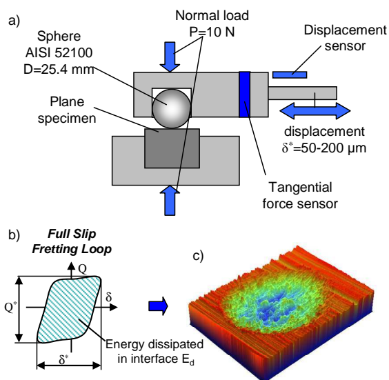
Fig. 1: Fretting test a) - contact configuration, b) - fretting loop, c) - fretting wear scar (Ti-6Al-4V).
