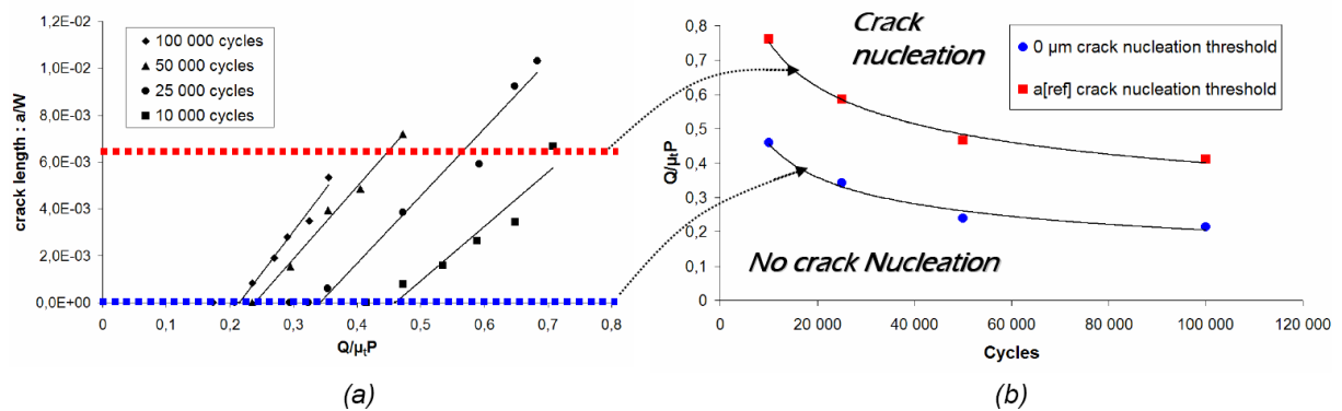
Figure 13: (a) Experimental results of crack length observed at a specific \{Q,N\} value, (b) Evolution of the critical tangential force Q_c to initiate fretting cracks ( 0 \mu\text{m} cracks or a_{\text{ref}} cracks) in relation to the number of cycles.
