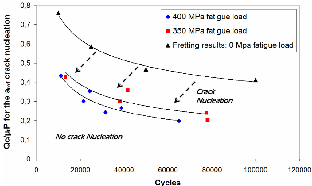
Figure 18: Tangential load threshold as a function of the number of cycle until obtaining the a_{\text{ref}} crack for fretting fatigue sollicitation: influence of the fatigue load.
