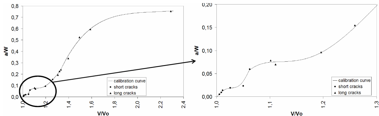
Figure 10: Fretting-fatigue Potential Drop Technique, empirical calibration curve for a cylinder on flat contact configuration, close-up for short cracks analysis.
