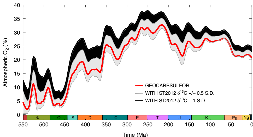
Fig. 5 Atmospheric O 2 sensitivity to changes in the \delta^{13}\text{C} record. The red line is our GEOCARBSULFOR model, the grey envelope is the atmospheric O 2 generated by \pm half a standard deviation change to the ocean-atmosphere \delta^{13}\text{C} record, based on the Saltzman and Thomas 48 data, and the black envelope is the +1 standard deviation
