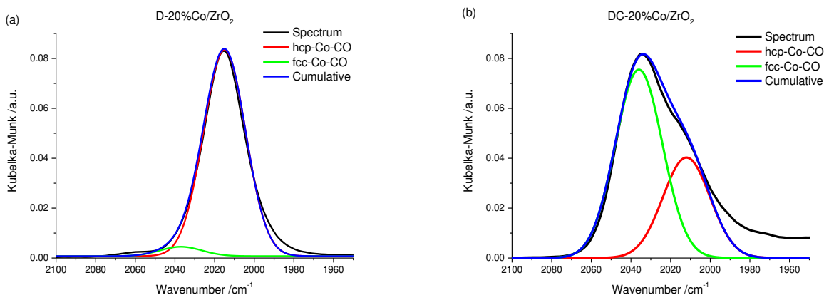
Figure 8. DRIFTS analysis of adsorbed CO onto D-20%Co/ZrO 2 (a) and DC-20%Co/ZrO 2 (b)
