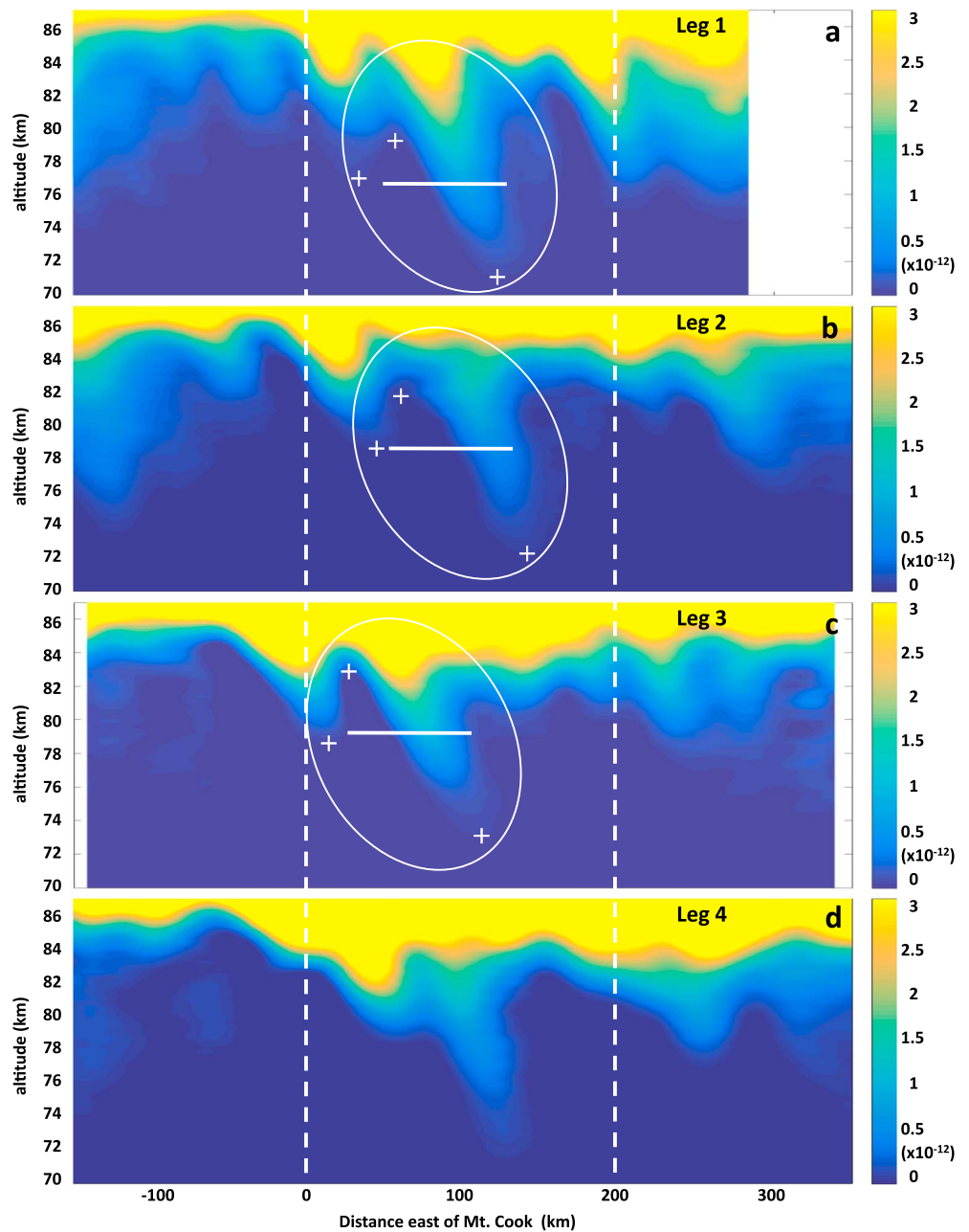
Figure 13. Estimated Na mixing ratios, R_{\text{Na}}(x,z) , at the bottom side of the Na layer for the four legs of RF22 (a–d). Note the peak-to-peak excursions exceeding \sim 10 km on each leg. White ovals and horizontal lines show the cases and central altitudes of the MW features used to compute local \langle u'w' \rangle estimates. The '+'s show the \zeta' extrema estimated from R_{\text{Na}} . Central times for the four flight legs were \sim 6:33 , 7:20 , 8:07 , and 8:52 UT. RF = Research Flight.
