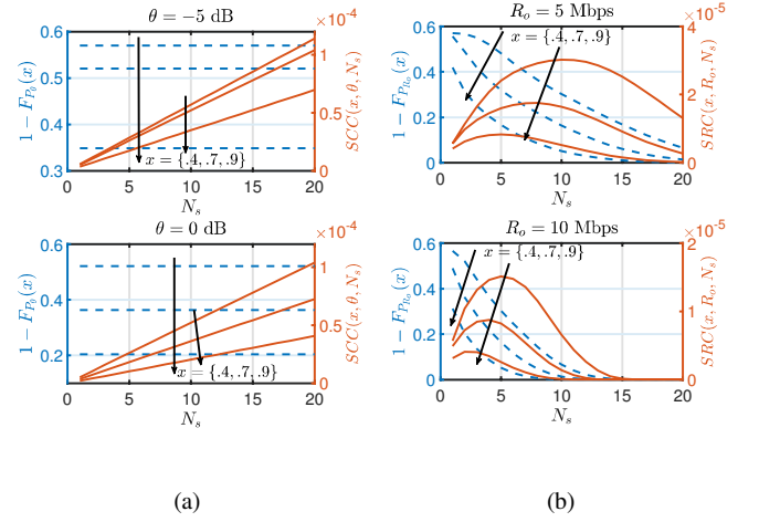
Fig. 5: (a) Meta-distribution (left axis- see (19)) and SCC (right axis - see (23)) against the number of channel partitions. (b) Meta-distribution (left axis- see (19)) and SRC (right axis - see (23)) against the number of channel partitions. All for UMi large-scale fading model, W = 20 MHz and for full load cell N_a = N_s .
