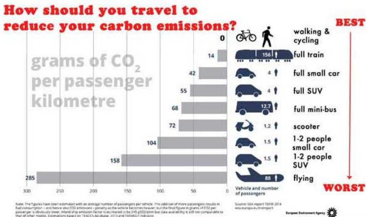
Figure 1: Grams of CO 2 e per passenger kilometre. Source: Thorpe (2016).
