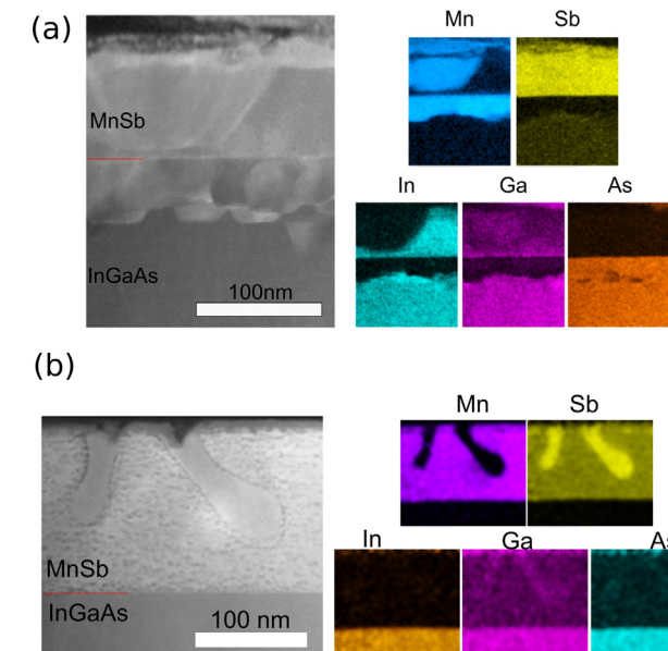
Fig. 5. Cross-sectional STEM and accompanying EDX maps taken from samples deposited with (a) J_{Sb/Mn} = 3.5 and T_{sub} = 415 \text{ }^\circ\text{C} (b) J_{Sb/Mn} = 9.5 and T_{sub} = 350 \text{ }^\circ\text{C} . The color intensity represents the elemental concentration, with black equating to none of the element being present. (For interpretation of the references to colour in this figure legend, the reader is referred to the web version of this article.)
