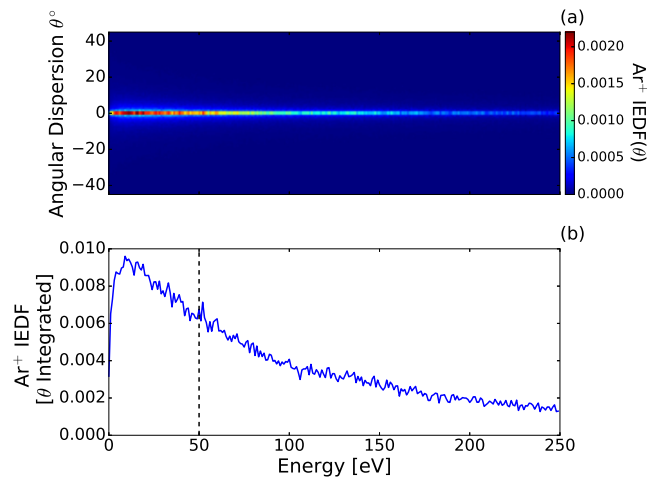
Figure 13: Phase-averaged (a) angularly resolved and (b) angle integrated Ar + ion energy distribution function adjacent to the powered electrode dielectric at region 2 ( R, Z = 2.1 \text{ mm}, 21 \text{ mm} ) for a 450 V \gamma -mode discharge. Plenum pressure 226 Pa, (1.7 Torr) argon, 13.56 MHz at 450 V, wall temperature 963 K
