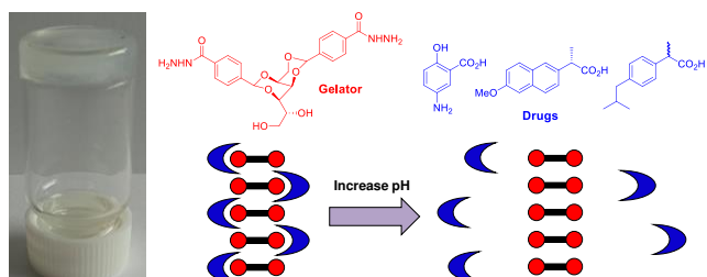
Figure 17. Image of hydrogel formed by DBS-CONH \text{NH}_2 and naproxen. Structures of the gelator and some acid-functionalised non-steroidal anti-inflammatory drugs. Schematic of pH mediated drug uptake and release as a result of interactions with the self-assembled nanofibre surfaces.
