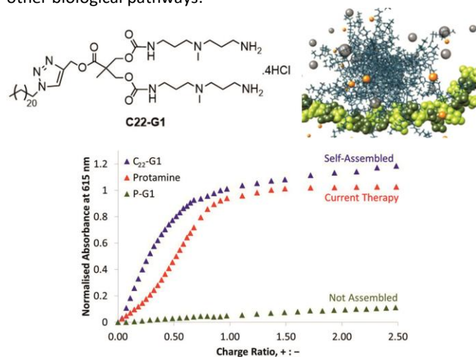
Figure 8. Structure of C 22 -G1, multiscale modelling simulation of C 22 -G1 self-assembled into a multivalent structure and bound to heparin, and binding study comparing the ability of C 22 -G1, current therapy protamine, and a non-self-assembling precursor (P-G1) indicating that in buffer, the self-assembling nanosystem outperforms protamine, and that there is a clear quantifiable SAMul binding effect.
