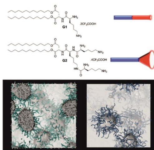
Figure 9. Compounds G1 and G2 have different hydrophobic/hydrophilic ratios and different molecular shapes, which give rise to self-assembled nanostructures with different morphologies – cylindrical micelles and spherical micelles respectively – as indicated by multiscale modelling.
