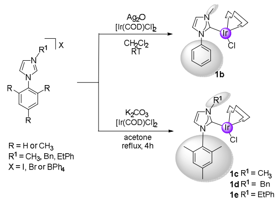
Scheme 3 Synthetic routes to 1 containing the specified C 2 -asymmetric carbene.
