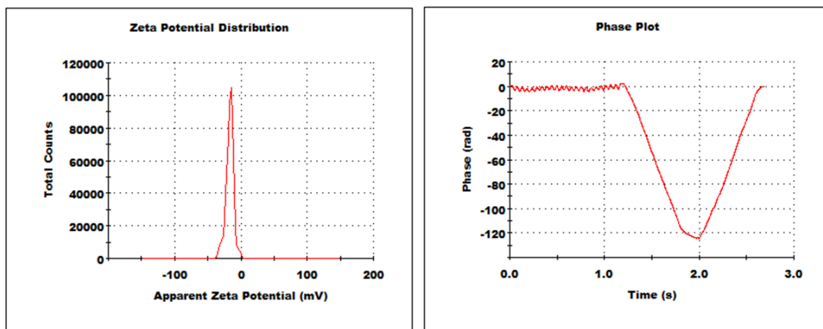
Figure S6. Representative graphs showing zeta potential distribution ( left ) and a ‘good quality’ phase plot ( right ) of Poly[(Lys(Cbz)LA) 26.6 - b -(Glu(Bz)LA) 28.3 ] dispersion at pH 11.2 (37 °C), suggesting that the particles are monomodal and stable (Data: n = 3). A viscosity of 0.891 cP, a dielectric constant of 78.6, and Henry function of 1.5 were used for the zeta potential calculations.
