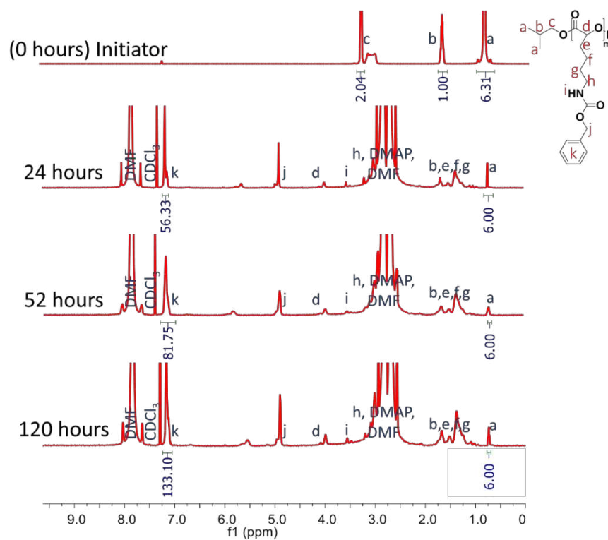
Figure S2. ^1H NMR spectra obtained from the analyses of reaction fractions that were extracted from the ROP of Lys(Cbz) OCA from an isobutanol molecule.
