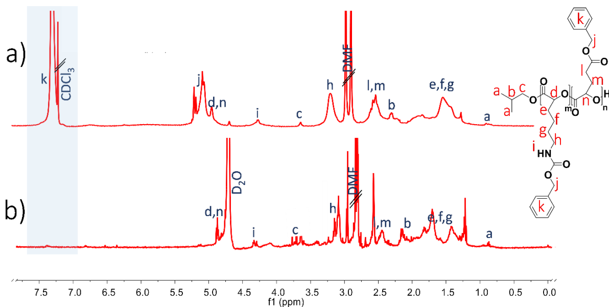
Figure S9. 1 H NMR spectra of (a) poly[(Lys(Cbz)LA) m -b-(Glu(Bz)LA) n ] prior to carrying out deprotection and (b) the deprotected poly[(LysLA) m -b-(GluLA) n ], revealing the absence of Cbz and Bz ester-protecting groups, which were removed by Pd/C catalytic hydrogenolysis.
