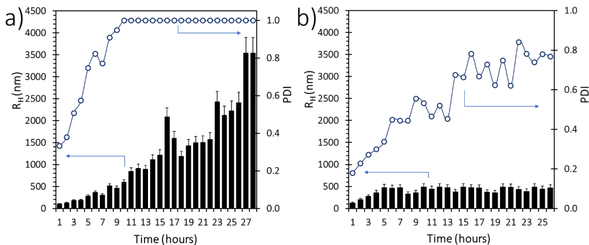
Figure S10. The evolution of the size of aggregates and the PDI values of poly[(LysLA) 26.6 -b-(GluLA) 28.3 ] NPs that were incubated at (a) pH 4.5, at 37 °C and at (b) pH 11.2, at 37 °C.
