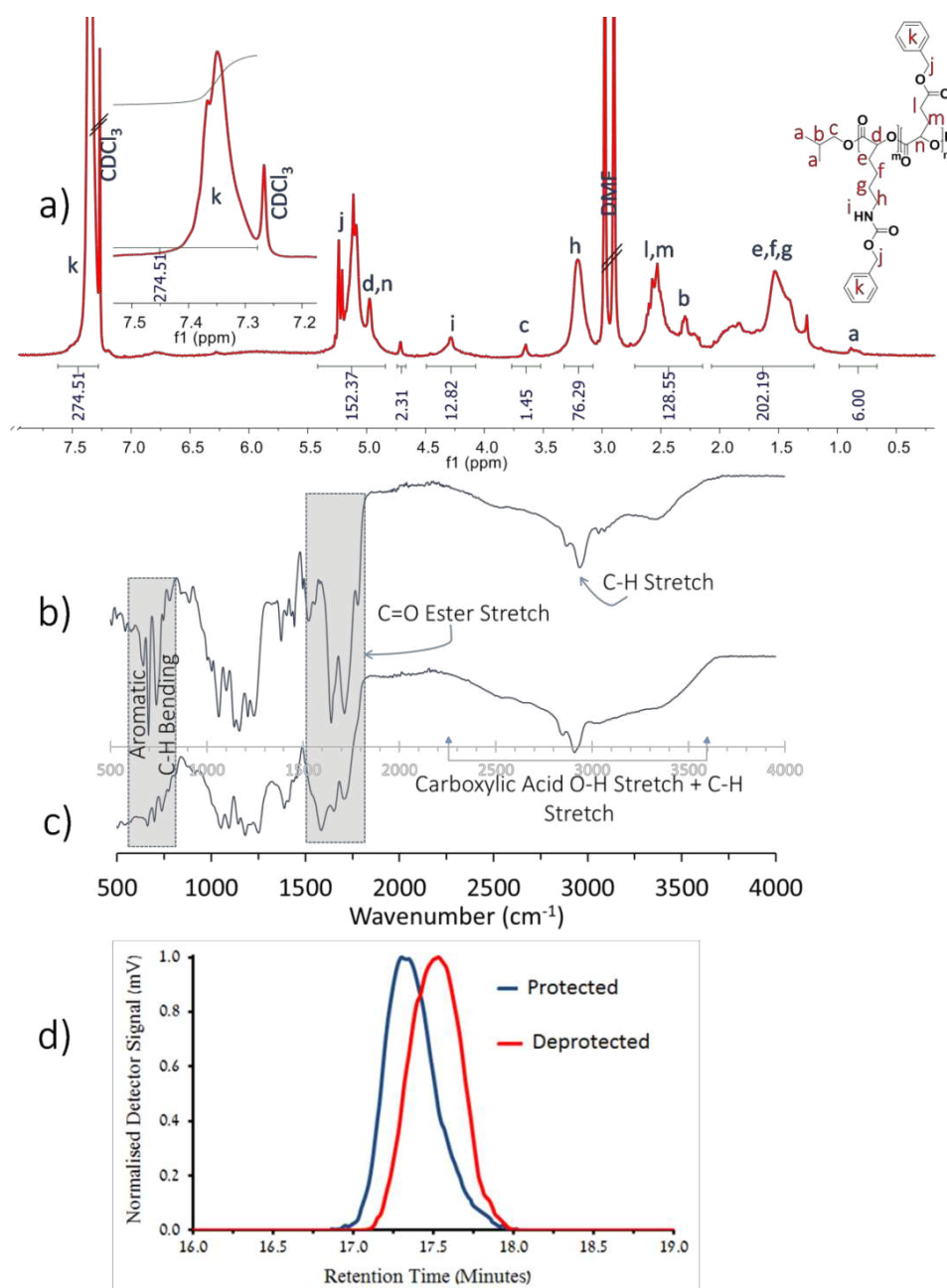
Figure S3. (a) ^1\text{H} NMR spectrum of poly[(Lys(Cbz)LA) _{26.6} - b -(Glu(Bz)LA) _{28.3} ], FTIR spectra of poly[(Lys(Cbz)LA) _{26.6} - b -(Glu(Bz)LA) _{28.3} ] before (b) and after poly(ester) deprotection (c), and (d) GPC chromatograms obtained from the analyses of poly[(Lys(Cbz)LA) _m - b -(Glu(Bz)LA) _n ] macromolecules before after poly(ester) deprotection and after poly(ester) deprotection.
