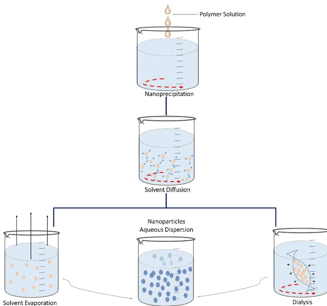
Figure S1. Illustration of the route to the generation of (nano)particles from poly(amino acid)-based macromolecules in solution, using the 'dropping-in' method.
