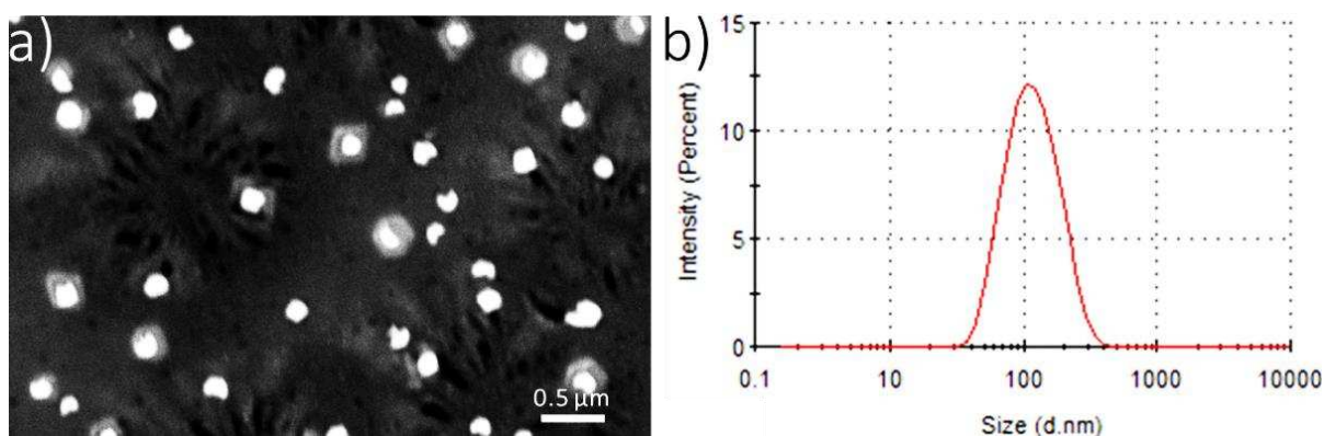
Figure S7. (a) SEM microphotograph and (b) DLS chart, revealing the size-distribution of Dox-loaded poly[(Lys(Cbz)LA) 26.6 - b -(Glu(Bz)LA) 28.3 ] NPs. Scale bar represents 0.5 μm.
