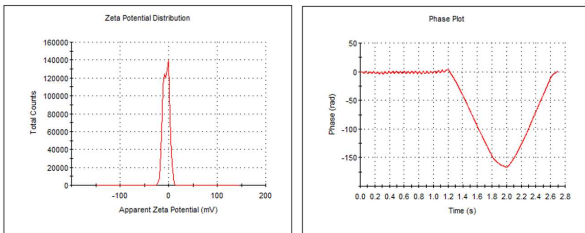
Figure S4. Representative graphs showing zeta potential distribution ( left ) and a 'good quality' phase plot ( right ) of Poly[(Lys(Cbz)LA) 26.6 - b -(Glu(Bz)LA) 28.3 ] dispersion at pH 4.2 (37 °C), suggesting that the particles are monomodal and stable (Data: n = 3). A viscosity of 0.891 cP, a dielectric constant of 78.6, and Henry function of 1.5 were used for the zeta potential calculations.
