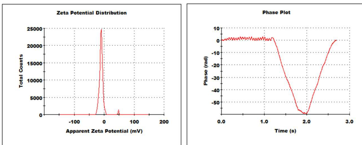
Figure S5. Representative graphs showing zeta potential distribution ( left ) and a 'good quality' phase plot ( right ) of Poly[(Lys(Cbz)LA) 26.6 - b -(Glu(Bz)LA) 28.3 ] dispersion at pH 7.4 (37 °C), suggesting that the particles are monomodal and stable (Data: n = 3). A viscosity of 0.891 cP, a dielectric constant of 78.6, and Henry function of 1.5 were used for the zeta potential calculations.
