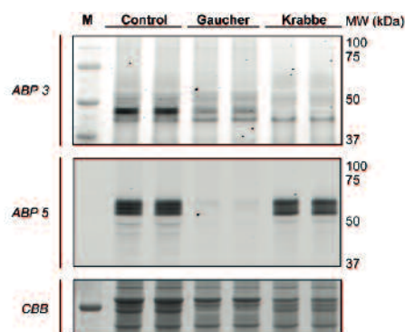
Figure 5. Labeling of Gaucher and Krabbe patient fibroblasts with ABPs 3 and 5. Fibroblasts from Gaucher and Krabbe disease patients, and healthy volunteer were lysed and incubated overnight with Concanavalin A beads for enrichment of glycosylated proteins. Bead-bound GALC was labeled with ABP 3 (1 \mu M) followed by labeling of GBA with ABP 5 (0.1 \mu M). Samples were resolved by 10% SDS-PAGE with fluorescent readout followed by Coomassie brilliant blue (CBB) staining. 'M': protein marker.
