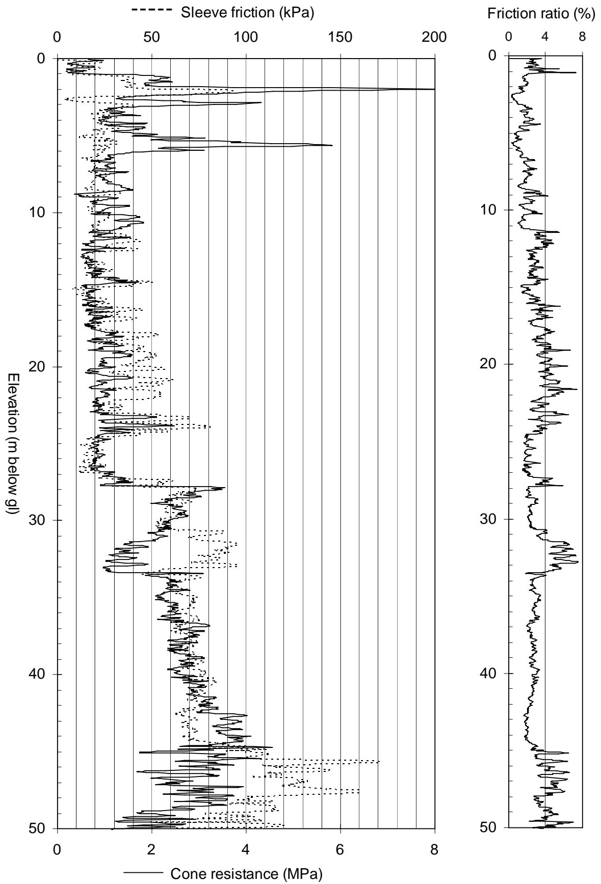
Figure 4: Data obtained from CPT6C
