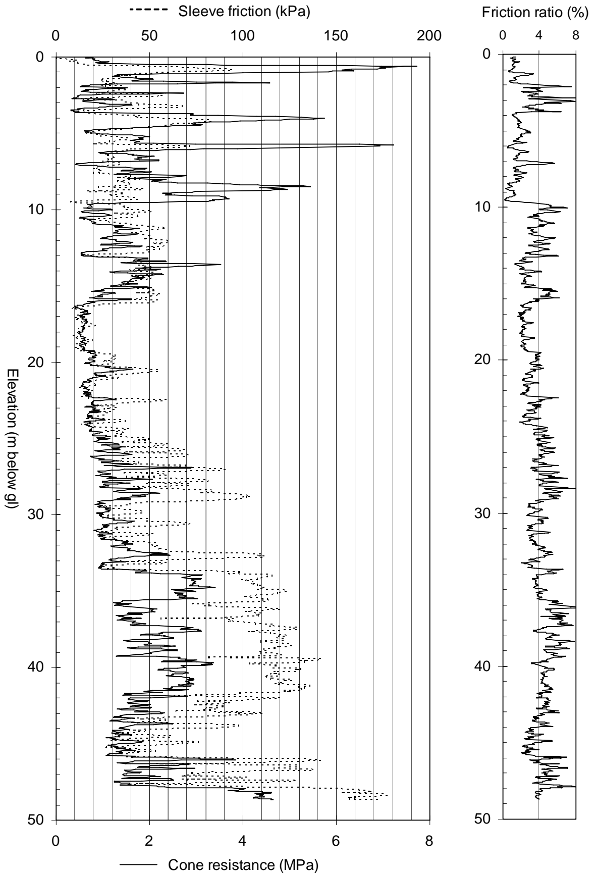
Figure 3: Data obtained from CPT4C
