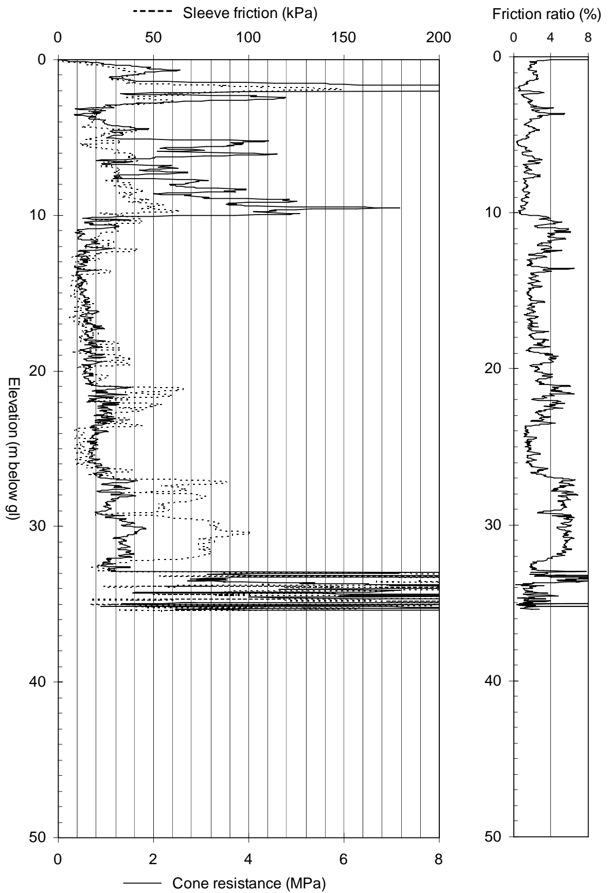
Figure 5: Data obtained from CPT7C
