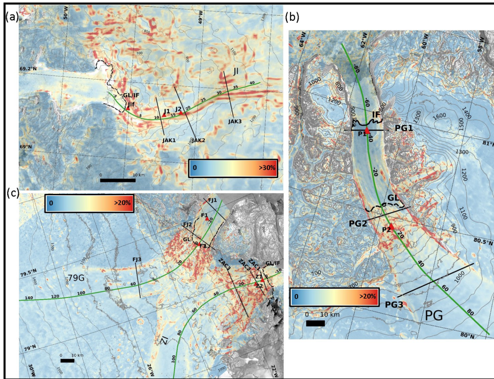
Figure 3. Time-averaged (2014–2017) uncertainty in ice velocity at each site expressed in percentage, based on the signal-to-noise ratio (SNR) for (a) JI, (b) PG, and (c) 79G and ZI.
