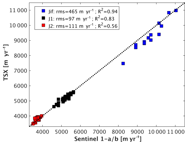
Figure 4. Comparison between co-located and contemporaneous Sentinel 1-a/b (6 to 12 days average) and TerraSAR-X (11 days average) Jakobshavn Isbræ velocity measurements at Jif, J1 and J2 locations (blue, black and red squares, respectively), together with root mean square (rms) and correlation coefficients ( R^2 ).
