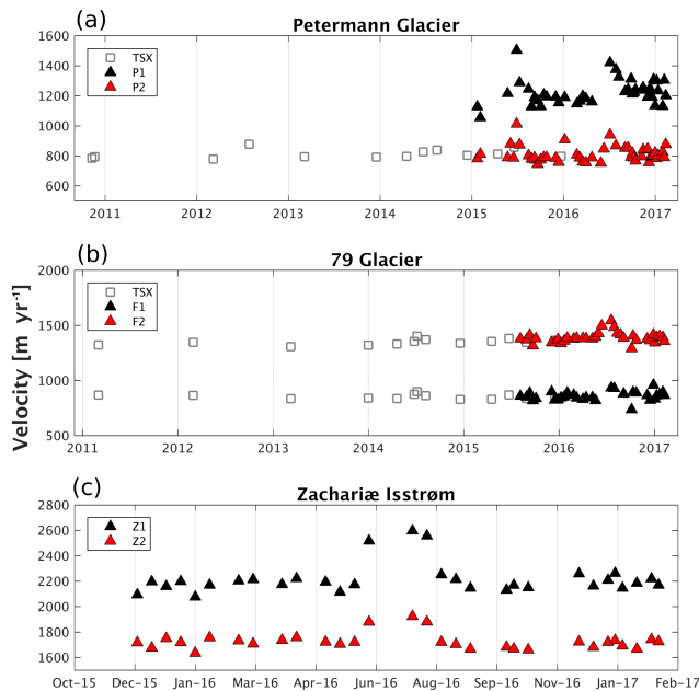
Figure 7. Temporal evolution of ice velocity at the locations indicated in Fig. 1 over (a) Petermann Glacier, (b) Nioghalvfjædsfjorden and (c) Zachariæ Isstrøm. The data derived from TerraSAR-X (11 days – Joughin et al., 2016) and Sentinel 1-a/b (6 to 12 days) are represented as grey squares and coloured triangles, respectively.
