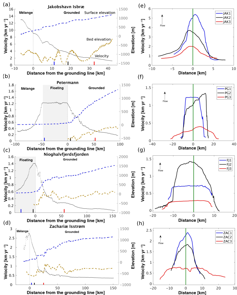
Figure 2. Average velocities (2014–2017) extracted from along- and across-flow profiles of Jakobshavn Isbræ, Petermann Glacier, Nioghalvfjærdsfjorden, and Zachariæ Isstrøm. Panels (a–d) present along-flow profiles of ice velocity (solid black lines), surface elevation from the GIMP DEM (Howat et al., 2014; dashed blue lines) and bed elevation from the IceBridge BedMachine Greenland V2 product (Morlighem et al., 2015; dashed yellow lines). The location of each profile is shown in Fig. 1 (green lines). The grey shaded area represents the floating regions, and the light grey dashed line the ice front positions. The blue, black, and red markers represent the locations of the across-flow profiles. (e–h) show the across-flow velocity profiles (solid white lines in Fig. 1), centred on the main profile (solid green line).
