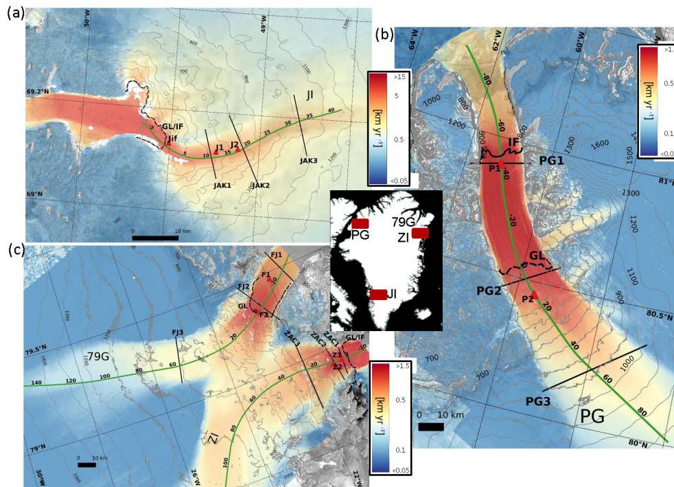
Figure 1. Time-averaged ice velocity magnitude maps for the period October 2014–February 2017: (a) Jakobshavn Isbræ (JI; 69° N, 50° W), (b) Petermann Glacier (PG; 81° N, 62° W), (c) Nioghalvfjærdsfjorden (79G; 79° N, 20° W), and Zachariæ Isstrøm (ZI; 78° N, 20° W) glaciers, derived from Sentinel-1 SAR images. Velocities are shown on a logarithmic scale and overlaid on a SAR backscatter intensity image and thin grey lines represent elevation. The along-flow profiles are indicated by solid green lines scaled in kilometres, the solid black lines show the cross-flow transects, the red triangles represent the locations at which velocity time series are extracted, and the thick solid and dashed black lines represent the ice front locations (IF) and the grounding lines (GL), respectively. The inset figures show the location of each glacier.
