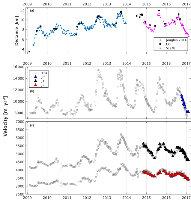
Figure 5. Temporal evolution of Jakobshavn Isbræ (a) ice front position extracted from Joughin et al. (2014), ESA Greenland Ice Sheet Climate Change Initiative (CCI) project (2017), and Sentinel-1a/b SAR images represented in blue, black, and magenta dots, respectively, where higher values correspond to ice front retreat. Changes in ice velocity through time is also shown (b, c), extracted at the locations indicated in Fig. 1. The velocity data derived from TerraSAR-X (11 days – Joughin et al., 2016) are shown as grey squares, and the data from Sentinel 1-a/b (6 to 12 days) as coloured triangles.
