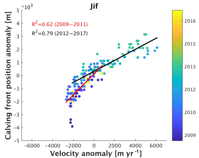
Figure 6. Comparison between Jakobshavn Isbræ ice velocity and calving front position anomalies at the Jif site, 0.8 km upstream of the calving front, between 2009 and early 2017. Positive values correspond to ice front retreat and speedup respectively. The red and black lines represent the linear regression through the 2009–2011 and 2012–2017 periods, respectively, together with the correlation coefficients ( R^2 ).
