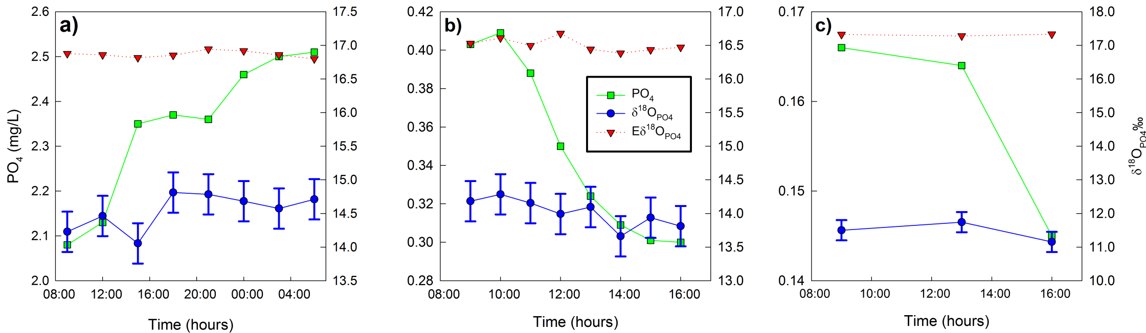
Figure 4. Time series data for PO 4 , δ 18 O PO4 and equilibrium (Eδ 18 O PO4 ) at 3 sites where different treatment technologies have been employed. (a) Site 14 disk filters only; (b) Site 15 disk filters and iron chloride; (c) Site 16 disk filters and aluminium sulphate
