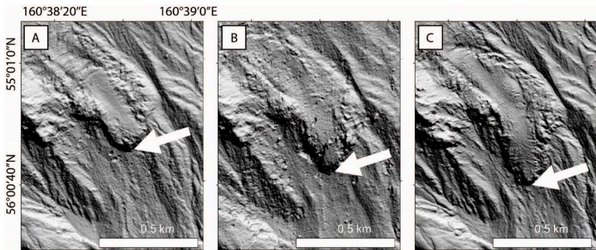
Figure 6. Evidence for terminus advance at Shmidta Glacier between (A) July 2012, (B) April 2014, and (C) October 2015 observed in the ArcticDEM 2m DSMs. The white arrow indicates the glacier terminus in each image. In total, the glacier advanced ~180 m over this period (~120 m between (A) and (B), and ~60 m between (B) and (C)). Location shown in Figure 5.
