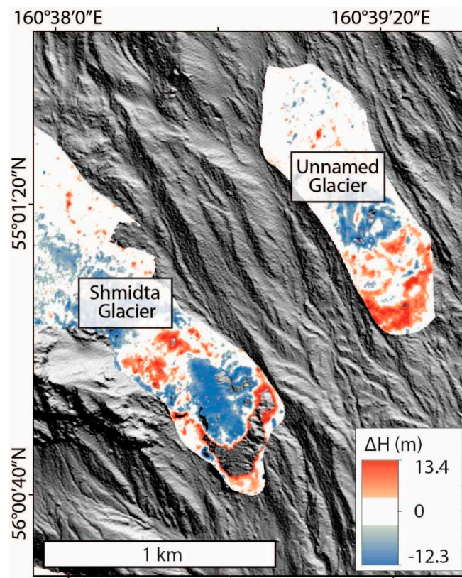
Figure 8. Surface elevation change between July 2012 and April 2014 (calculated from Arctic DEM 2 m DSMs) for the terminus of Shmidta Glacier and an adjacent unnamed glacier (white areas show where the surface elevation change is within measurement error). Location shown in Figure 5.
