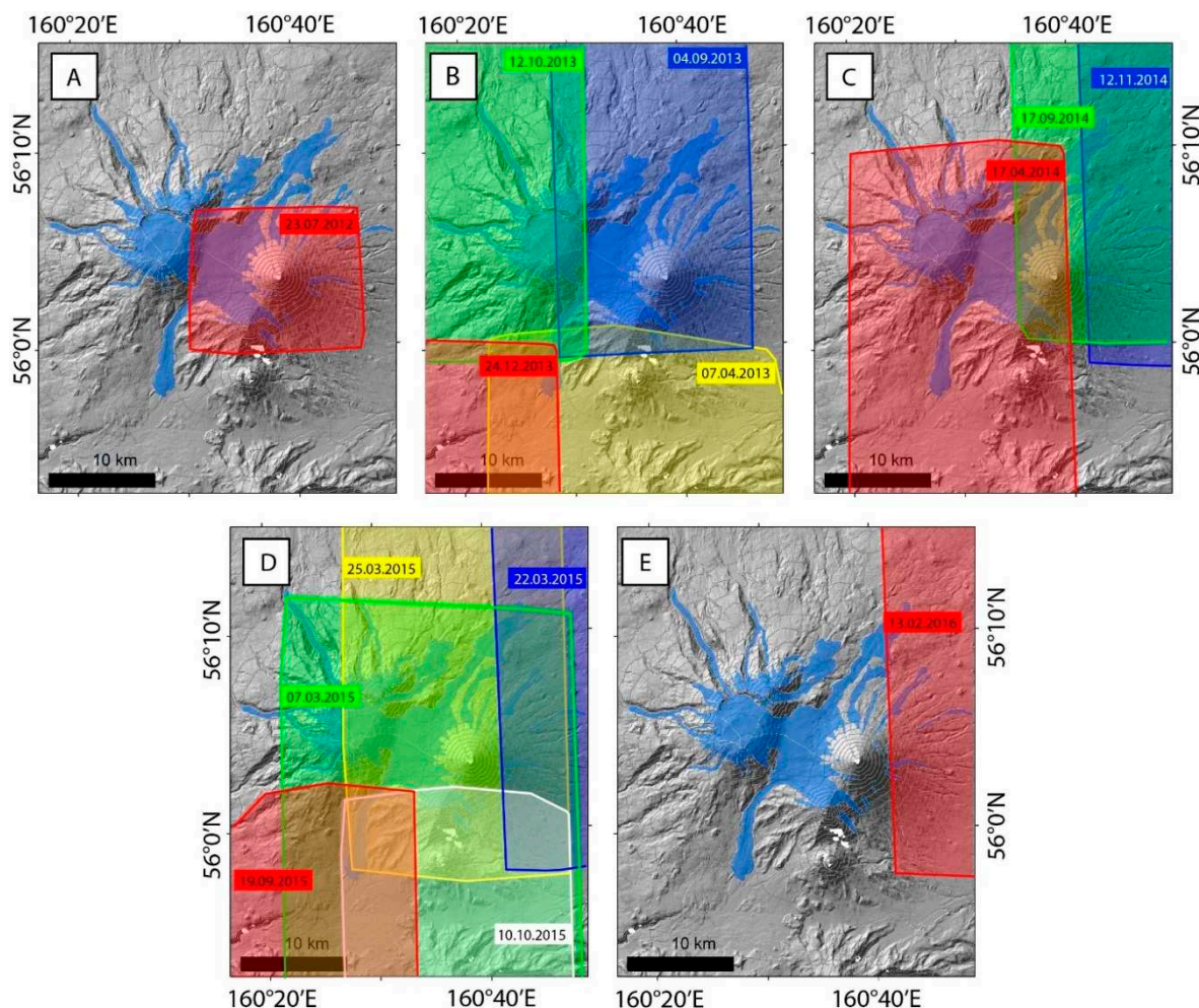
Figure 2. Coverage of the ArcticDEM 2m digital surface model (DSM) strips for the NKVG. (A) 2012. (B) 2013. (C) 2014. (D) 2015. (E) 2016. Mapped glaciers are shown (in blue) in the background image. Strip details are presented in Table 2.
