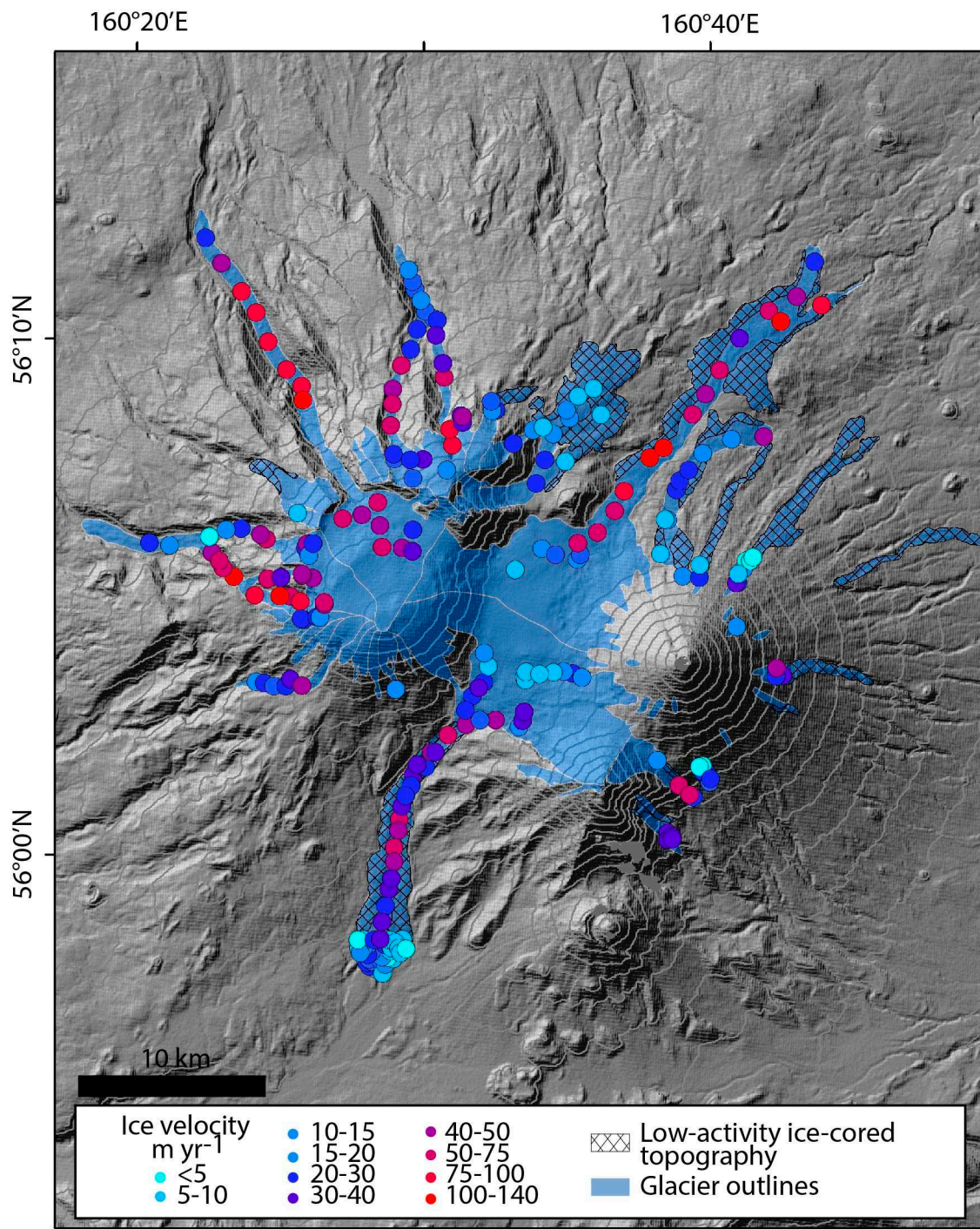
Figure 9. Estimates of annual glacier surface velocity in the NKVG during the period 2012–2015 based on ArcticDEM data.
