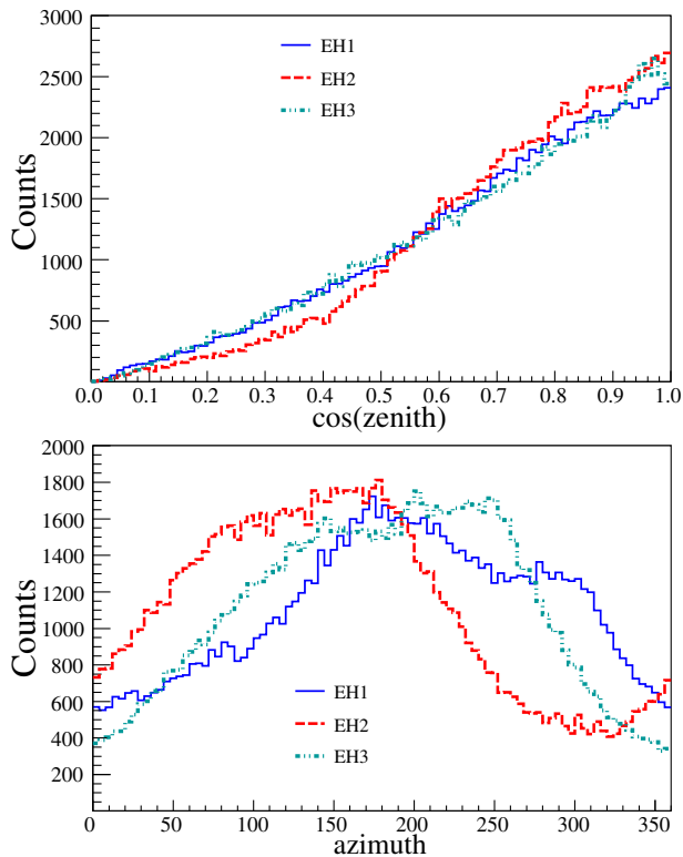
FIG. 4. Simulated trajectories of muons that reach the underground halls. By definition, zenith is the angle from the vertical and azimuth is the horizontal compass angle from true North. (A zenith angle of 0^\circ represents a downward-going muon, and an azimuthal angle of 0^\circ corresponds to a muon coming from the northern direction.) Differences in angular distributions at each hall are due to the mountain profile.
