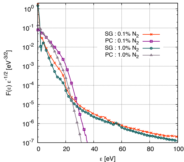
Figure 10. Electron energy distribution functions at 70 ns, at the spatial positions (a) x = 0.02 mm (corresponding to sheath – negative glow boundary, "SG") and (b) x = 0.60 mm (which belongs to the positive column, "PC"). The temporal and spatial window for the data collection are, respectively, \pm 1 ns and \pm 0.01 mm. Results are shown for 0.1% and 1.0% N_2 concentrations, at p = 1 bar, L = 1 mm, V_0 = 1000 V, \tau_p = 30 ns, and n_0 = 1.5 \times 10^{11} \text{cm}^{-3} (with VUV photons considered).
