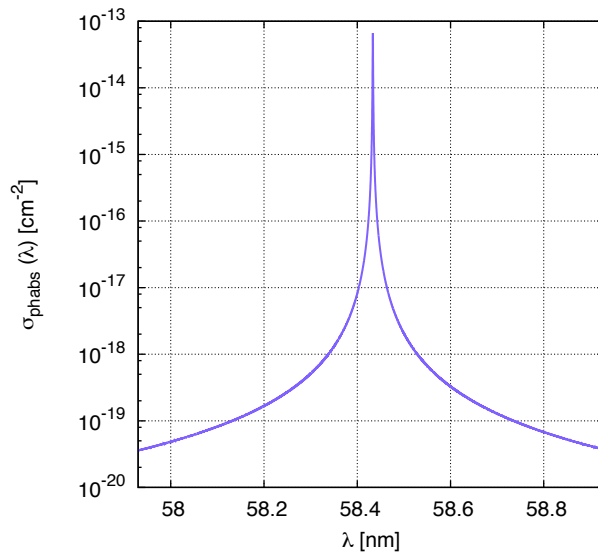
Figure 1. Photoabsorption cross section for the He 2^1\text{P} \rightarrow 2^1\text{S} resonance radiation.
