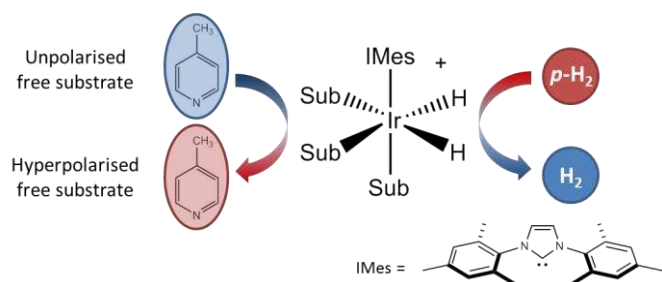
Figure 1 An active SABRE catalyst reversibly binds both p -H 2 and a substrate to allow polarization transfer from p -H 2 to the substrate in a polarization transfer field (PTF) of a few tens of gauss.
