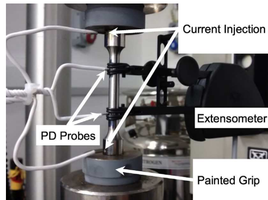
Fig. 2. Uniaxial tensile test experimental setup.
