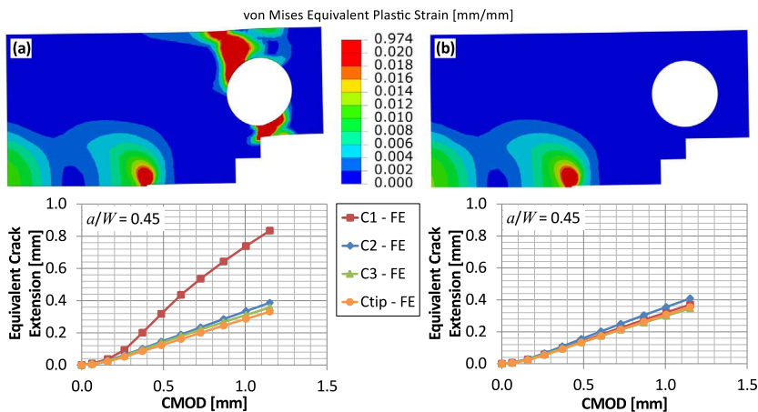
Fig. 18. Plastic strain distribution and equivalent crack extension due to strain for (a) FE model with rigid pin, (b) FE model with kinematic coupling boundary condition.
