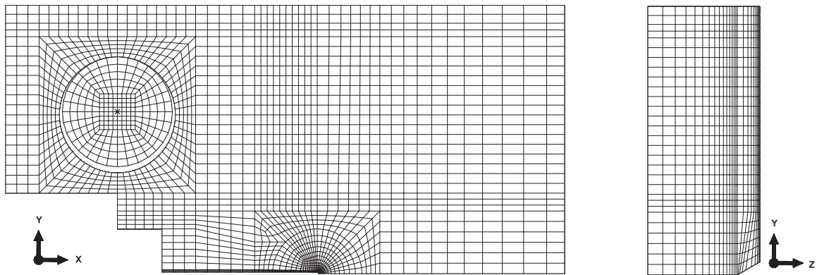
Fig. 10. FE mesh for C(T) specimen CTP_CT45 ( a/W = 0.45 ).
