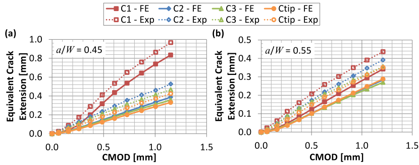
Fig. 17. Equivalent crack extension due to strain for C(T) specimens with different PD configurations and (a) a/W = 0.45 , and (b) a/W = 0.55 .
