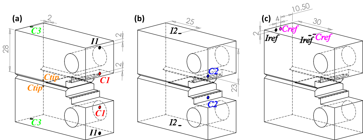
Fig. 8. C(T) specimen PD configurations.
