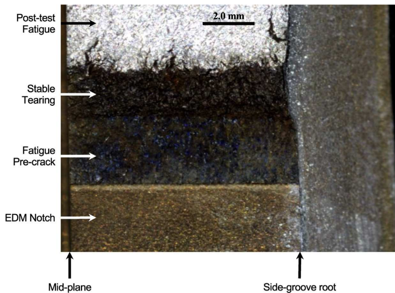
Fig. 22. Post-test fracture surface for specimen JIC_CT01.
