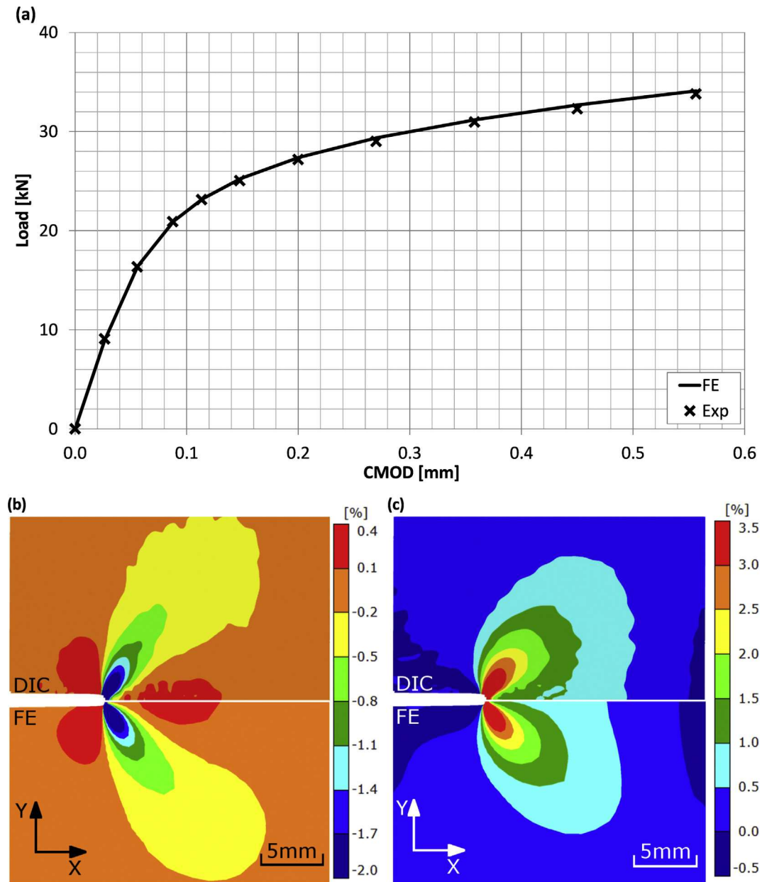
Fig. 11. Experimental validation of the SEN(T) structural FE model for specimen CTP_ST30 ( a/W = 0.3 ) showing (a) load-displacement plot, (b) \epsilon_{xx} and (c) \epsilon_{yy} .
