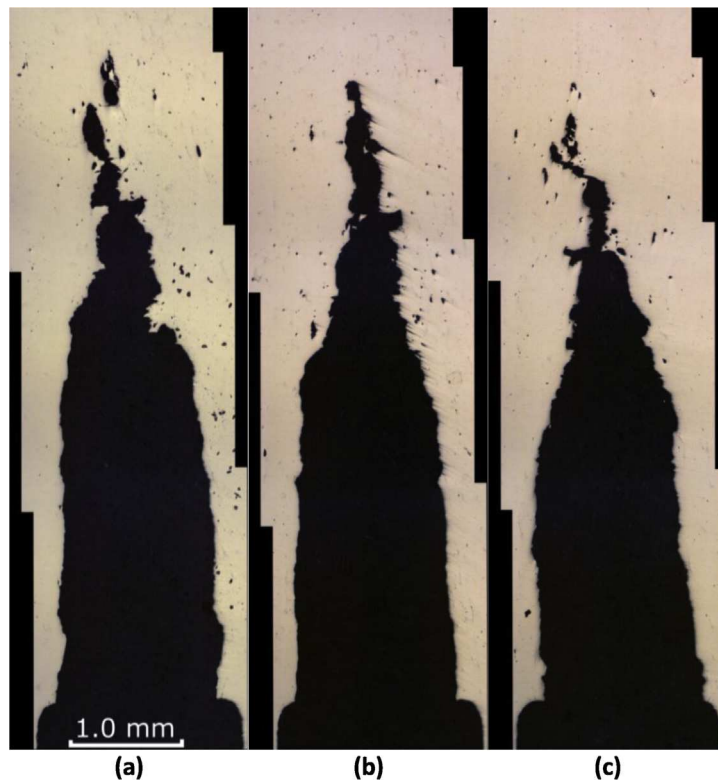
Fig. 21. Crack profiles at (a) mid-plane, (b) 2.5 mm from mid-plane, and (c) 5.0 mm from mid-plane.
