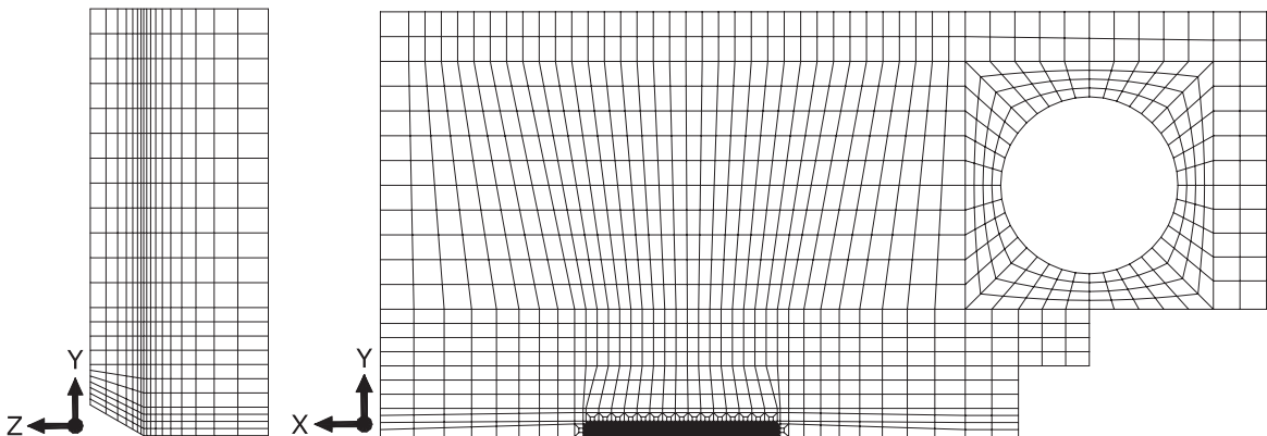
Fig. 24. FE mesh for modelling stable tearing in a C(T) specimen.
