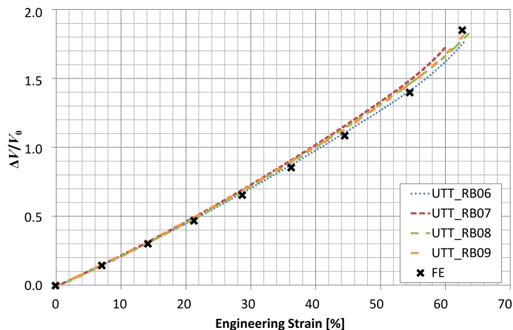
Fig. 6. Comparison of the relative change in PD for specimens UTT_RB06 to UTT_RB09 and the FE predictions.
