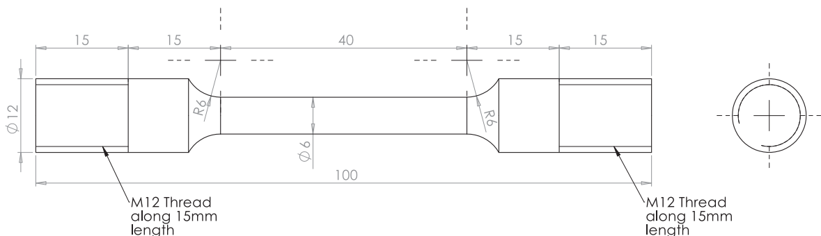
Fig. 1. Uniaxial tensile specimen geometry.
