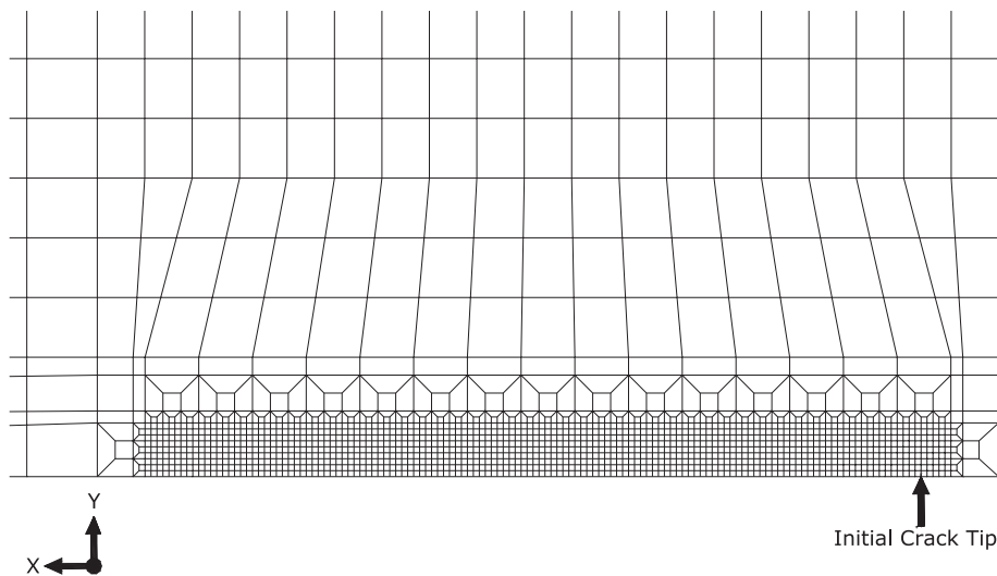
Fig. 25. Refined crack tip FE mesh for modelling stable tearing in a C(T) specimen.
