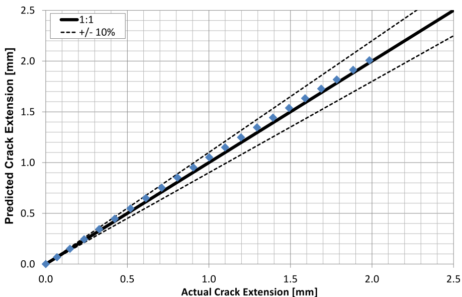
Fig. 27. Comparison of the modelled crack extension and the crack extension predicted from the FE PD predictions.
