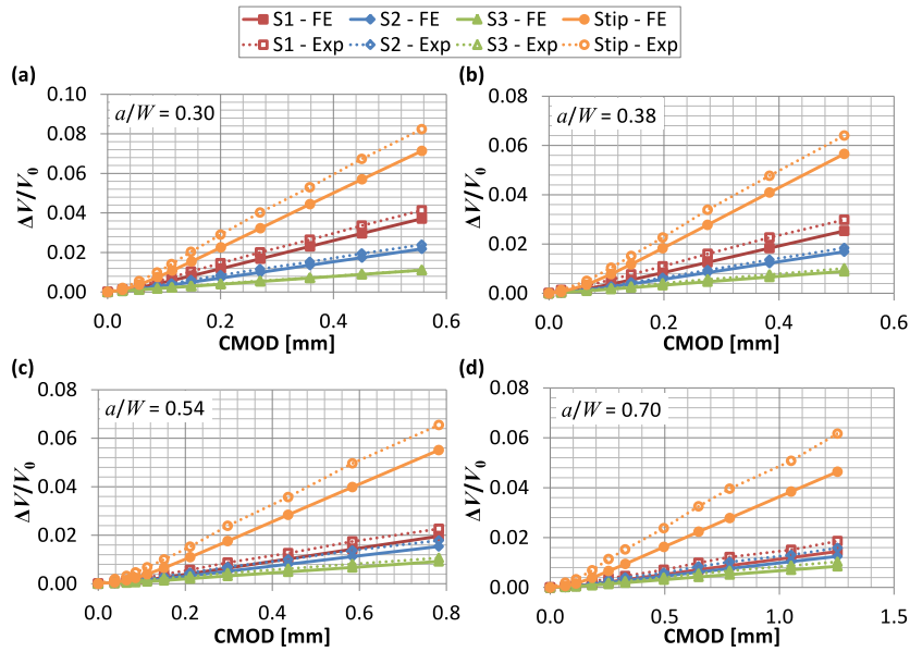
Fig. 12. Relative change in PD due to strain for SEN(T) specimens with different PD configurations and (a) a/W = 0.30 , (b) a/W = 0.38 , (c) a/W = 0.54 and (d) a/W = 0.70 .
