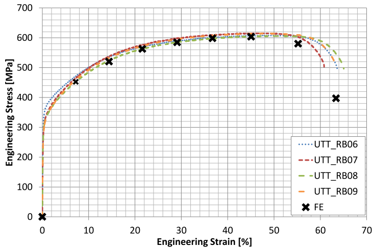
Fig. 5. Comparison of the engineering stress-strain data for specimens UTT_RB06 to UTT_RB09 and the FE predictions.
