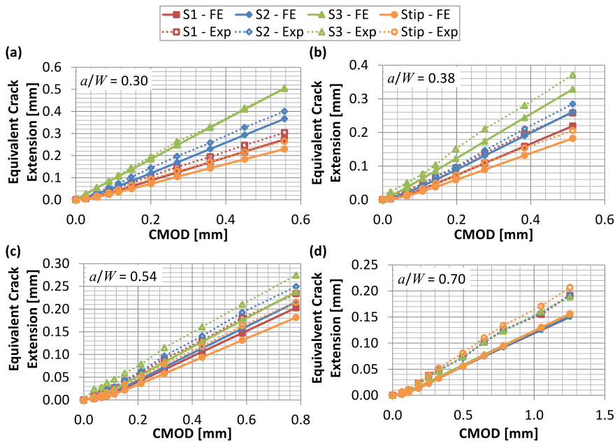
Fig. 13. Equivalent crack extension due to strain for SEN(T) specimens with different PD configurations and (a) a/W = 0.30 , (b) a/W = 0.38 , (c) a/W = 0.54 and (d) a/W = 0.70 .
