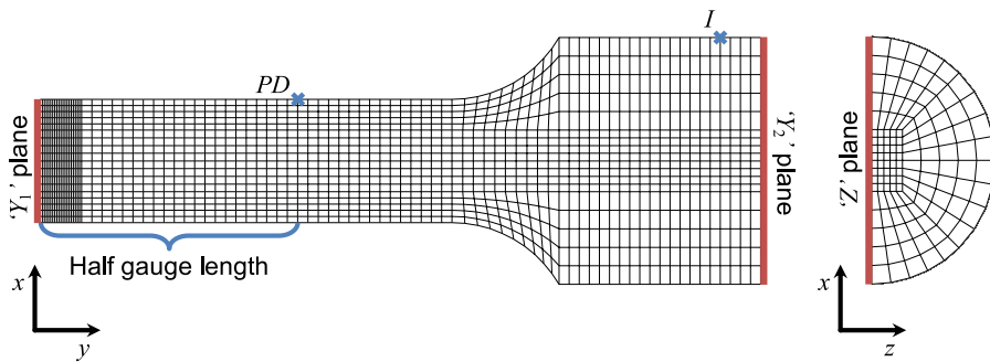
Fig. 4. Uniaxial tensile specimen FE mesh.
