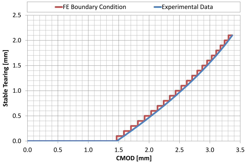
Fig. 23. Experimentally determined relationship between stable tearing and CMOD and the corresponding boundary condition applied to the FE model.
