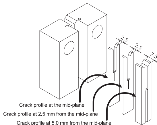
Fig. 20. Post-test sectioning of specimen JIC_CT01 to reveal the crack profile at the mid-plane and at 2.5 mm and 5.0 mm from the mid-plane.
