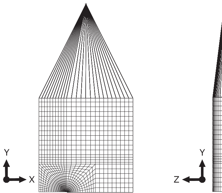
Fig. 9. FE mesh for SEN(T) specimen CTP_ST30 ( a/W = 0.30 ).
