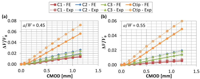
Fig. 16. Relative change in PD due to strain for C(T) specimens with different PD configurations and (a) a/W = 0.45 and (b) a/W = 0.55 .
