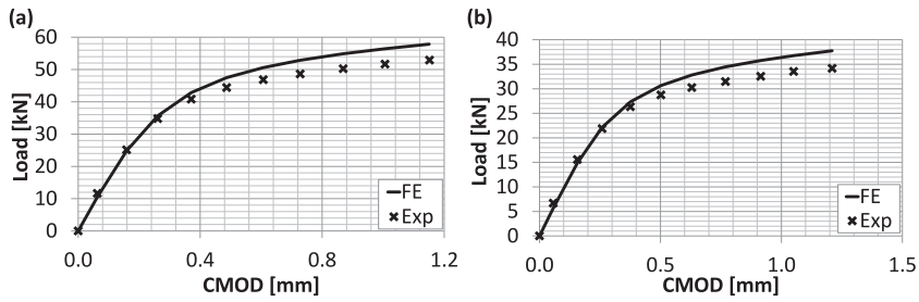
Fig. 14. Comparison of the experimental and FE load-displacement plot for C(T) specimens (a) a/W = 0.45 and (b) a/W = 0.55 .
