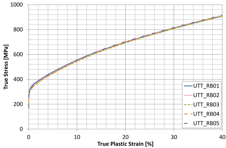
Fig. 3. True plastic stress-strain data for austenitic Type 316H stainless steel at room temperature.
