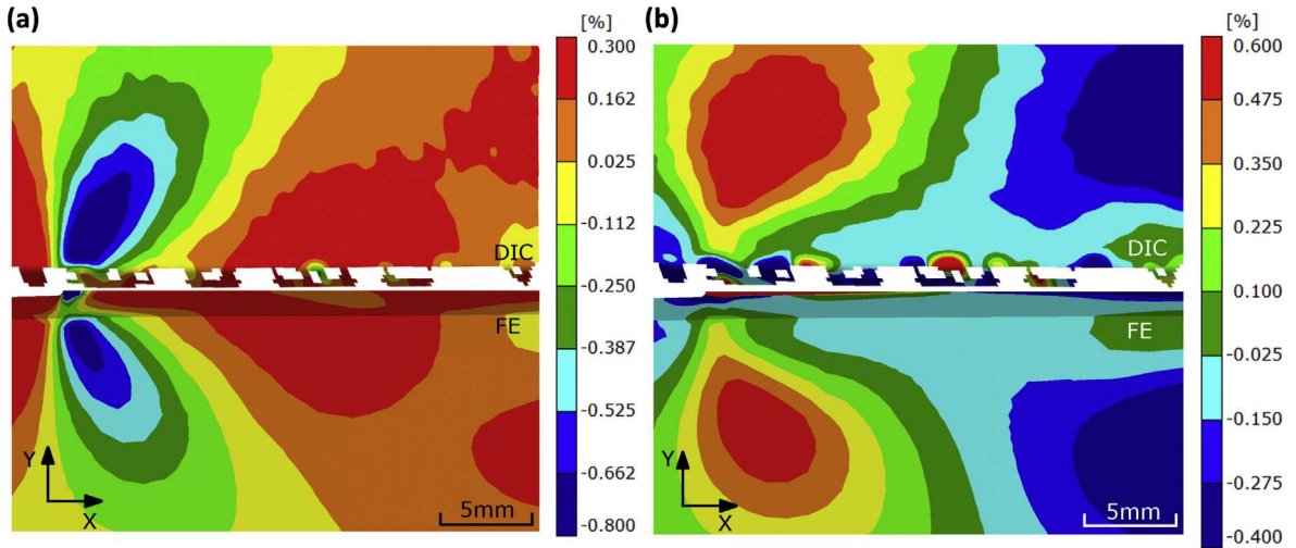
Fig. 15. Comparison of the experimental and FE surface strain field for the final displacement increment of specimen 04CTP_CT45 ( a/W = 0.45 ) showing (a) \epsilon_{xx} and (b) \epsilon_{yy} .
