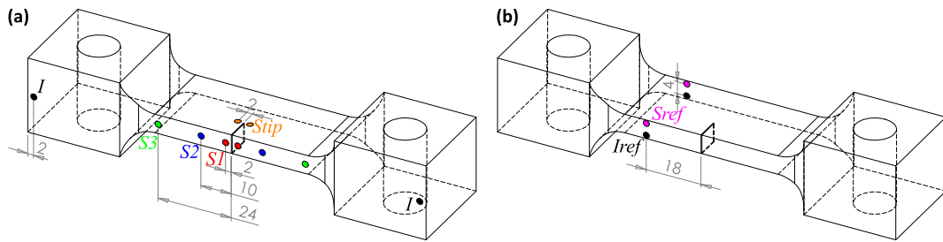
Fig. 7. SEN(T) specimen PD configurations.
