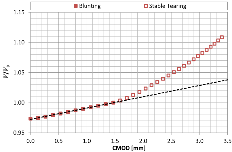
Fig. 26. PD vs. CMOD data predicted from the FE analysis.
