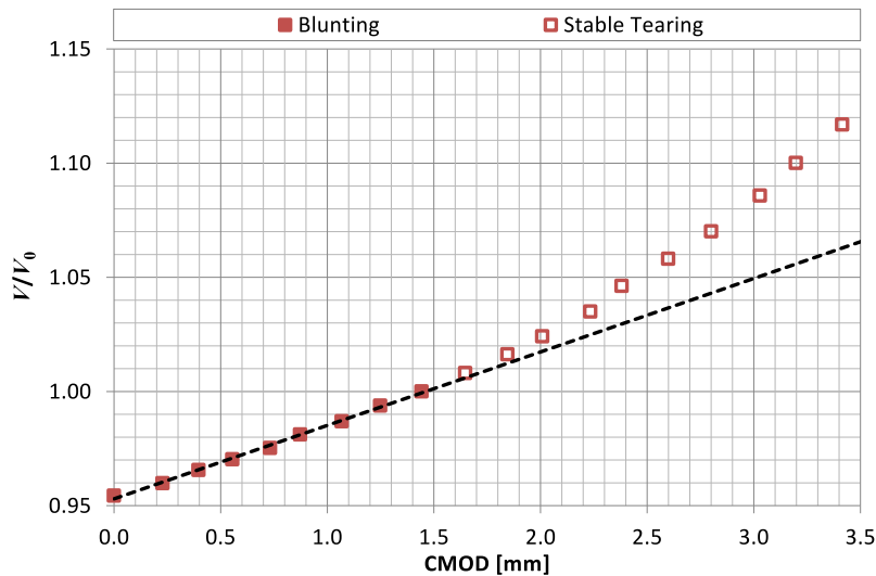
Fig. 19. Experimental PD vs. CMOD data.
