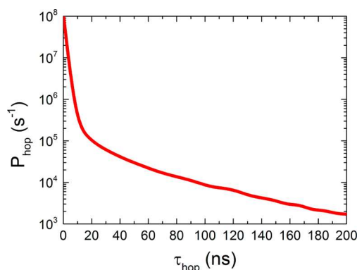
Figure 7. The probability density function for the site-to-site hopping times of charges in a fiducial simulation of F = 10^7 \text{V m}^{-1} and k_r = 10^7 \text{s}^{-1} . Although hop times covering 13 orders of magnitude are recorded, only a selection are shown here as the majority occur within 10 ns.
