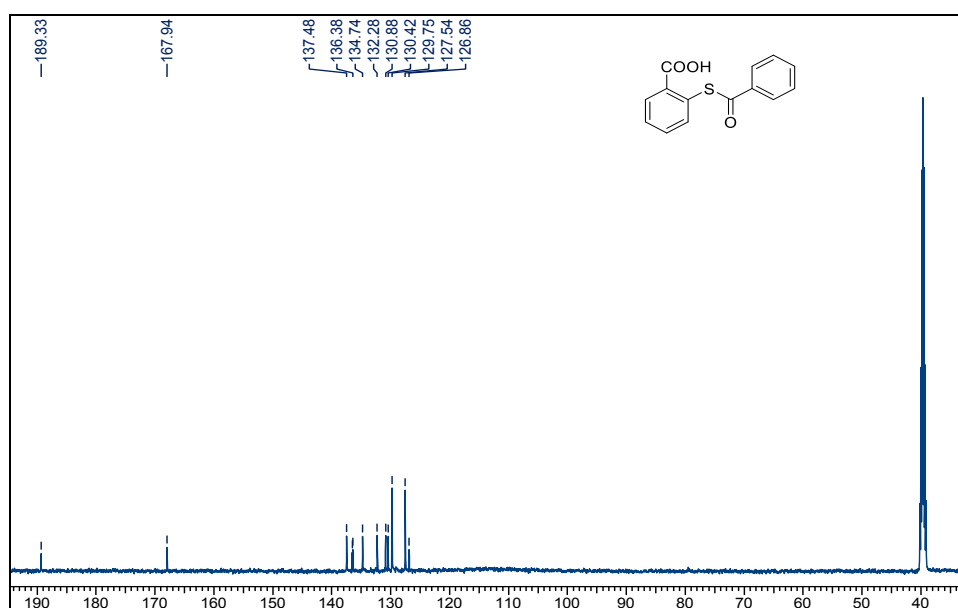
Fig. S 15: ^{13}\text{C} NMR spectrum of 2-(benzoylthio)benzoic acid in \text{DMSO-}d_6
