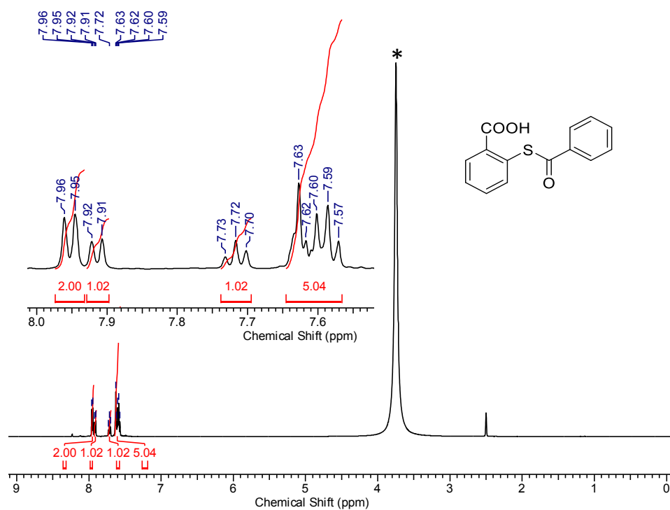
Fig. S 14: ^1\text{H} NMR spectrum of 2-(benzoylthio)benzoic acid in \text{DMSO-}d_6 . (* \text{H}_2\text{O} ).
