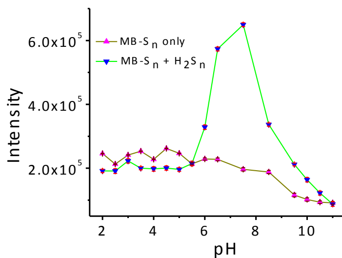
Fig. S 6: Emission response of MB-S n (10 μM) at different pH in the absence or presence of Na 2 S 2 (10 μM). λ EXT = 530 nm.
