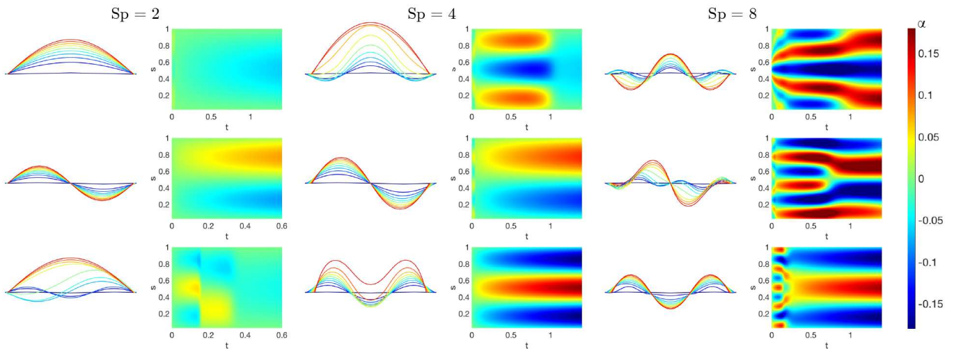
FIG. 4. Visualization of the buckling phenomenon for three different sperm numbers ( Sp=2 on the left, Sp=4 on the middle and Sp=8 on the right). Here N = 36 and k = 1.5 . The filament is displayed at regular intervals of time, coloured from blue (beginning) to red (end). Three different initial conditions lead to different outcomes. The colormap graphs show time on the x-axis and link number (discrete arclength) on the y-axis. The colours show the curvature (angles) over time, from blue for a highly negative curvature to red for a highly positive one. The filament quickly takes a waveform with fewer waves as time goes on. The higher the sperm number is, the longer it takes for the waves to vanish (note that the total time on the graphs is longer as the sperm number increases).
